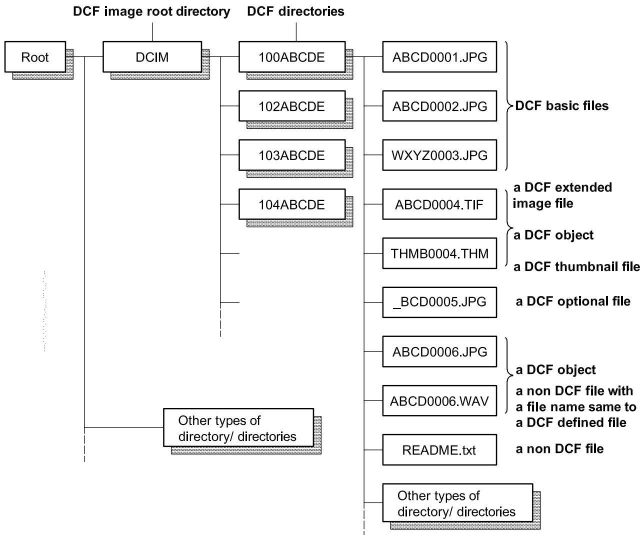
Figure D.1 — Typical filing system structure in DCF directories
