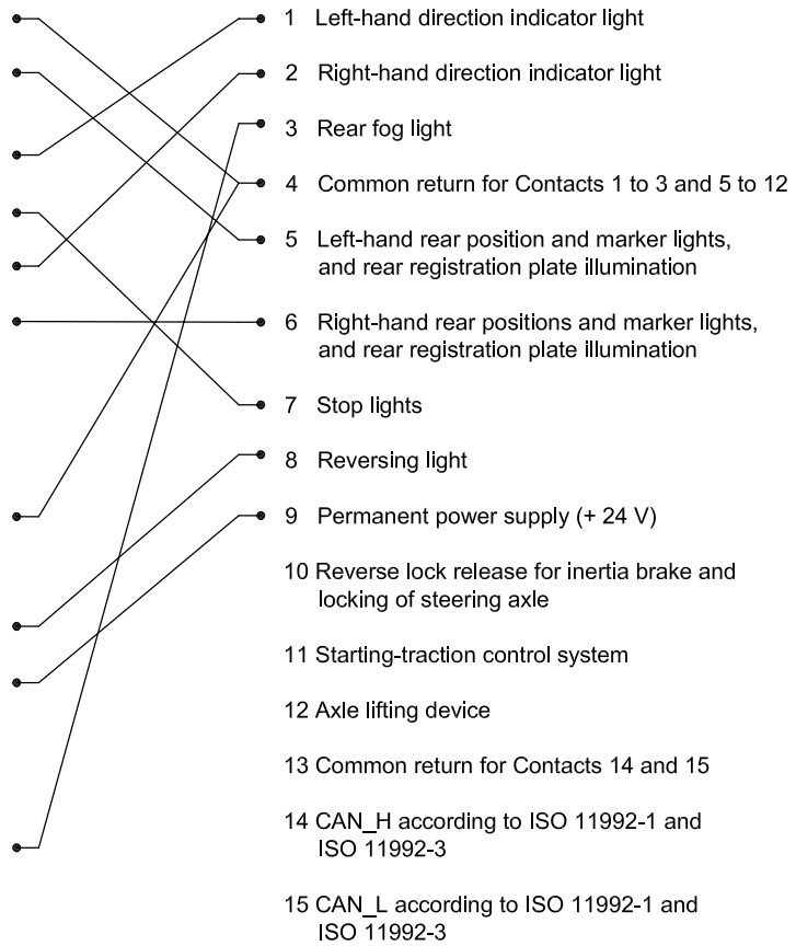
Figure A.3 — Internal wiring — Type B adapter (see Figure A.1)
