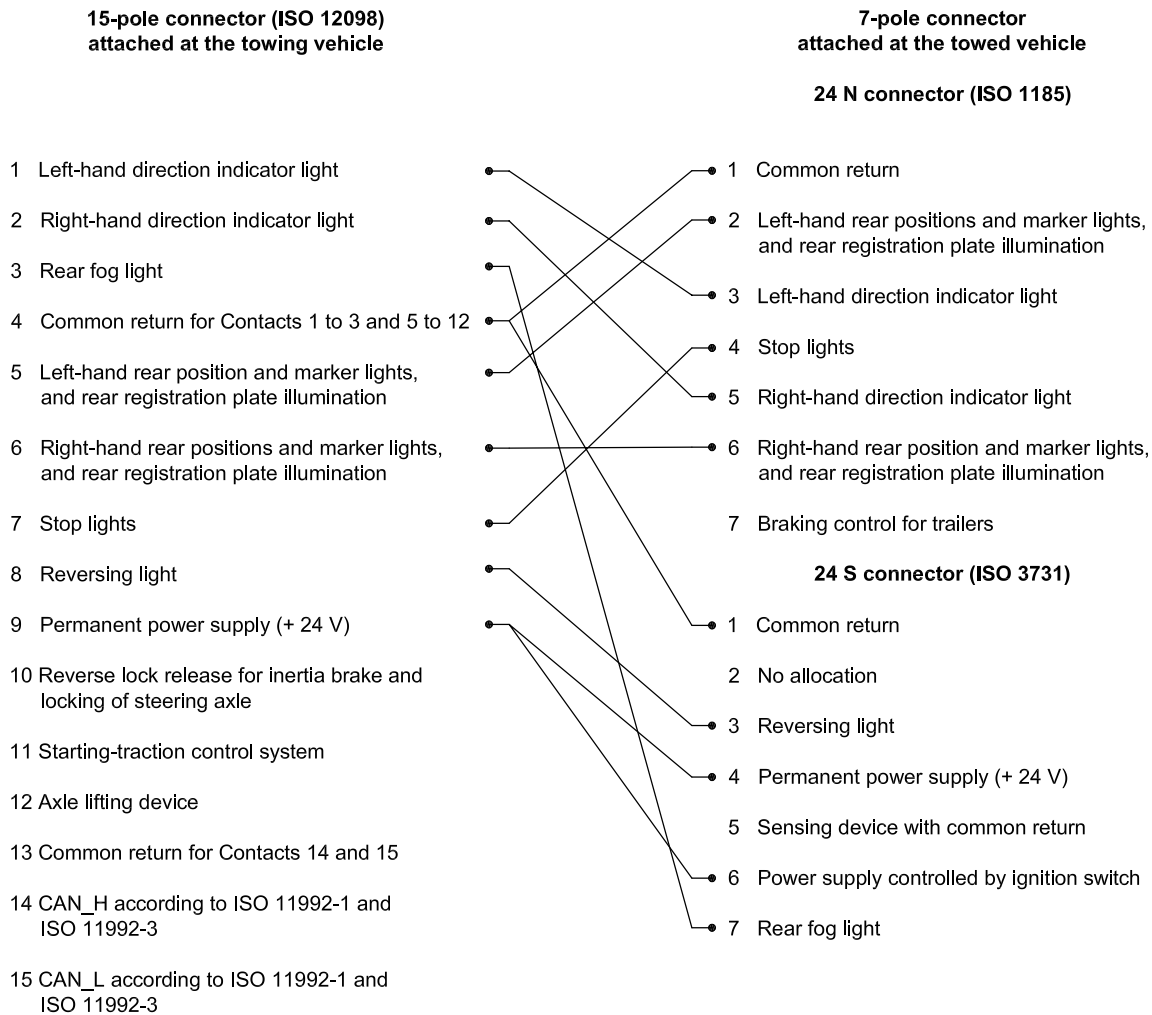
Figure A.2 — Internal wiring — Type A adapter (see Figure A.1)
