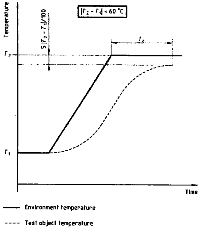
Figure A.2 — Temperature build-up time t_0 for |T_2 - T_1| < 60 \text{ }^\circ\text{C}
