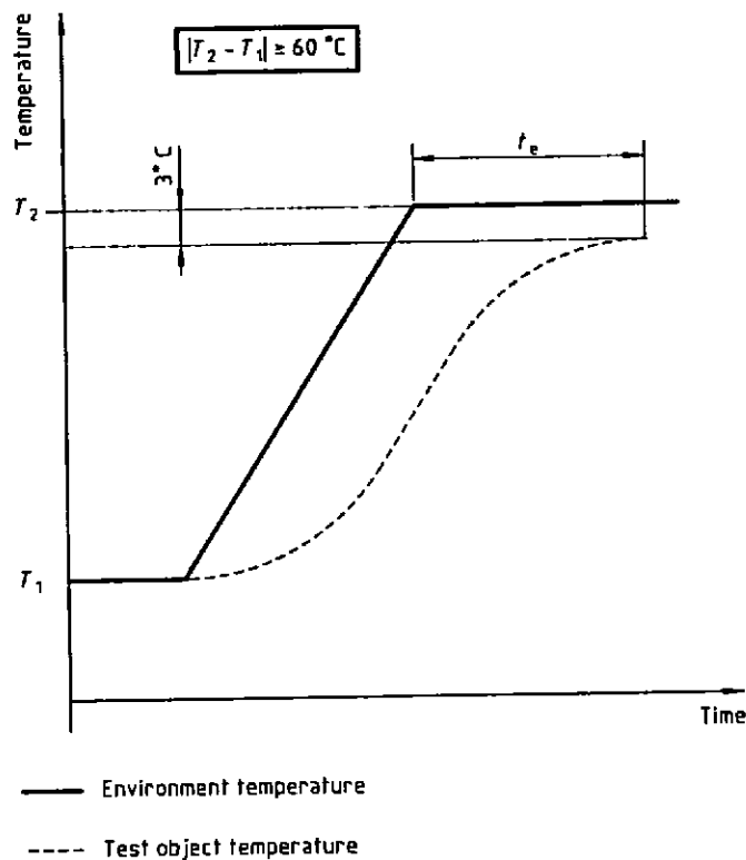
Figure A.1 — Temperature build-up time t_e for |T_2 - T_1| \geq 60 °C
