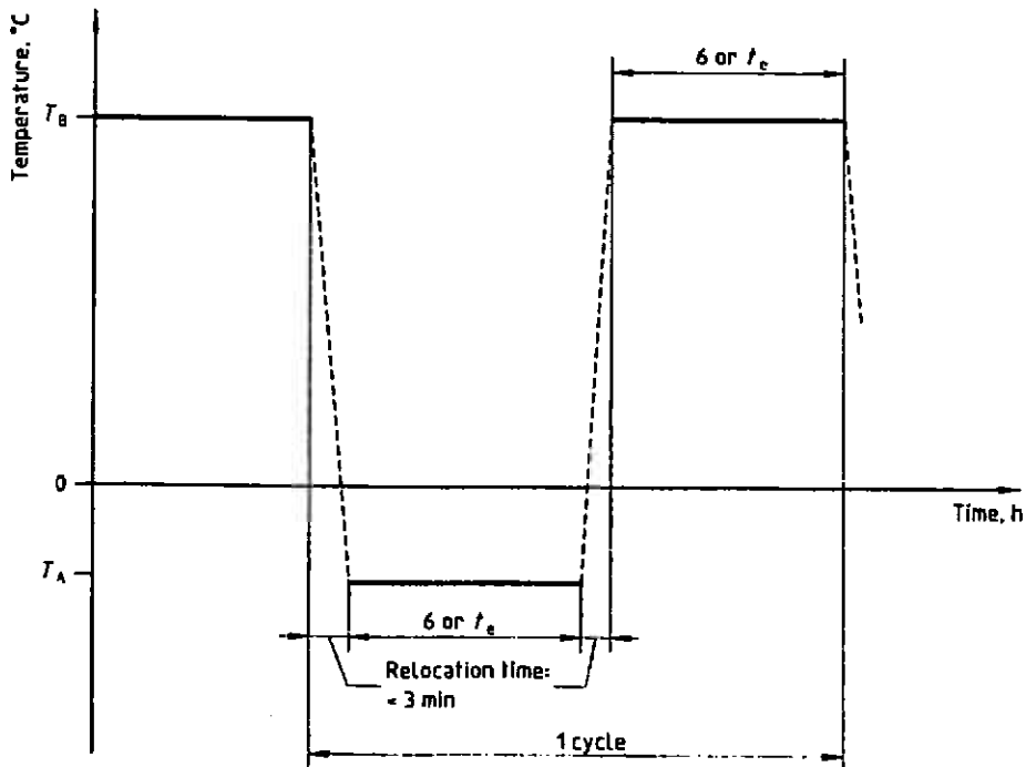
Figure 11 — Cycle of temperature shock test
