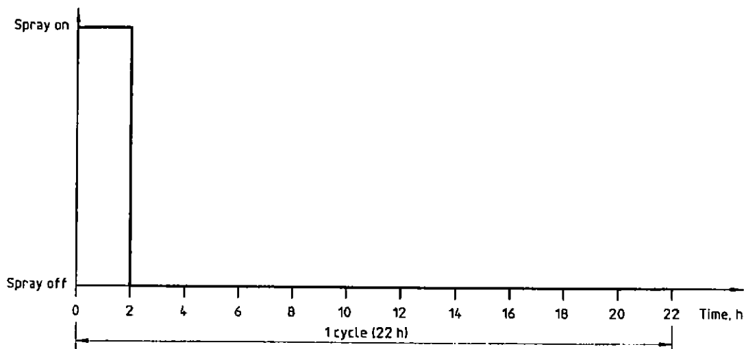
Figure 9 — Salt spray cycle
