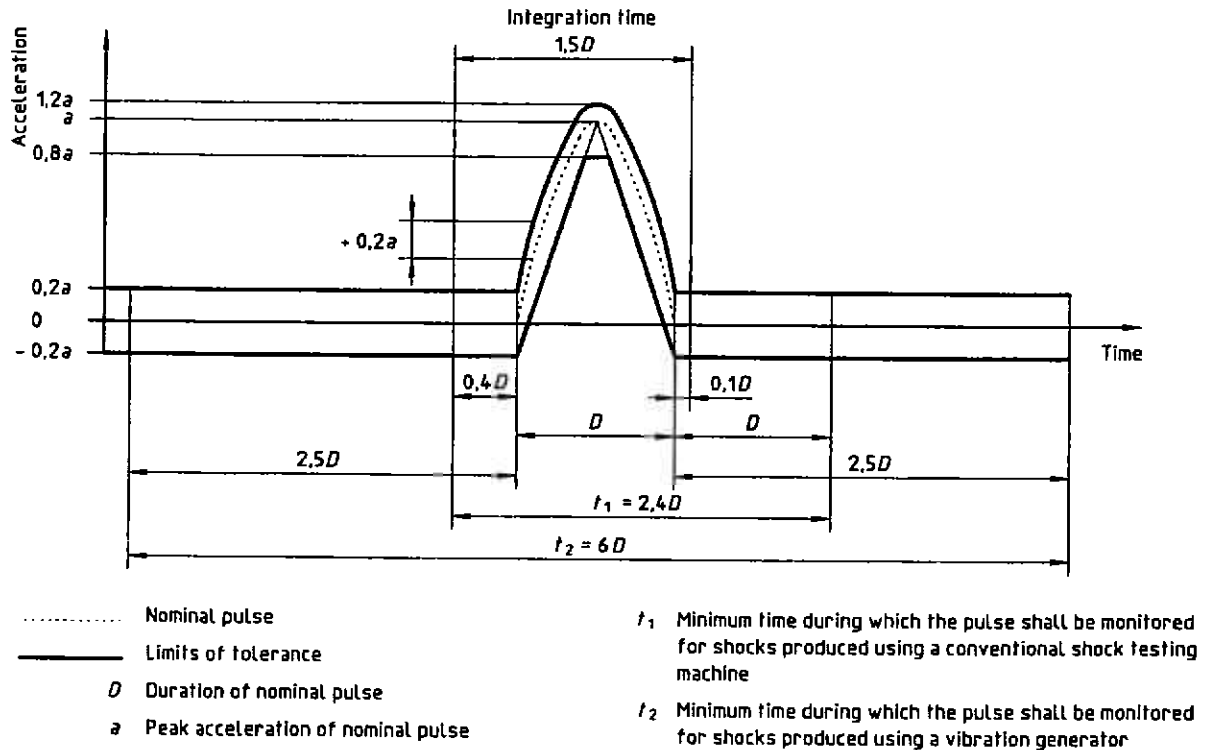
Figure 3 — Half-sine pulse
