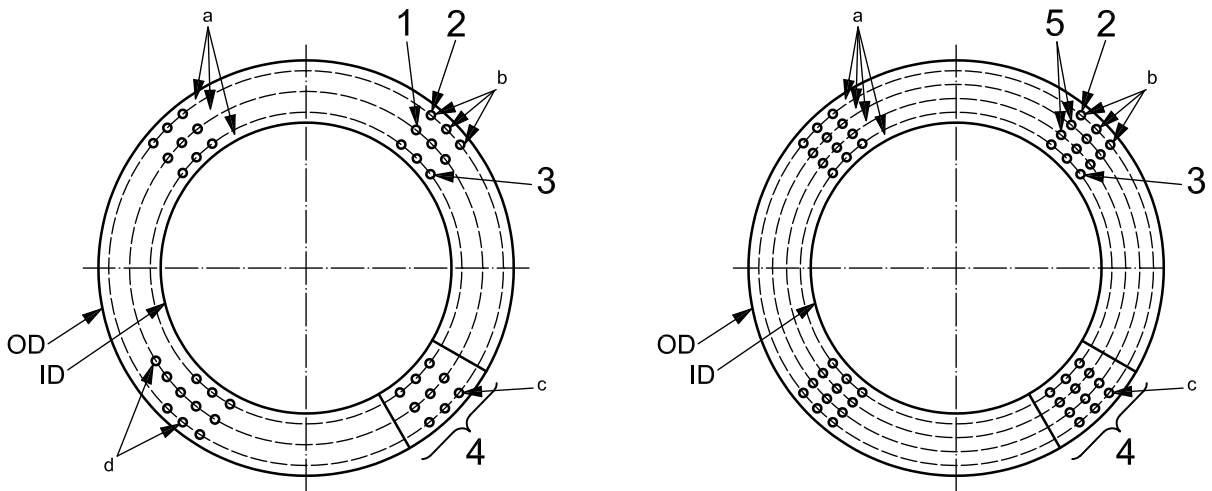
a) Thickness < 50 (< 2)
