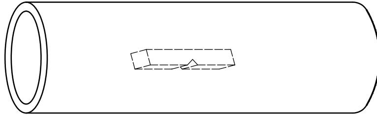
a) Drill-pipe body — Charpy specimen
