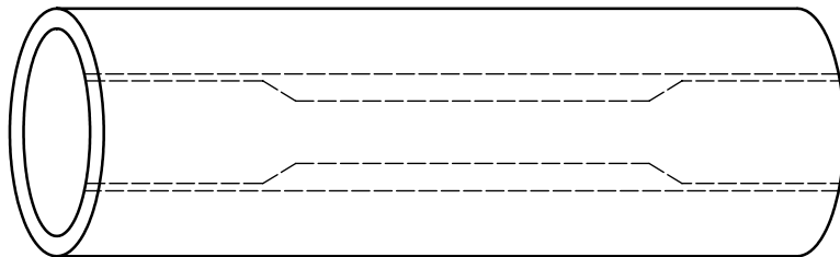
c) Drill-pipe-body tensile — Strip specimen
