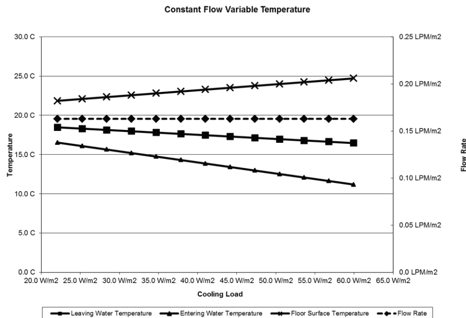
Figure A.2 — Constant flow variable supply water temperature control strategy
