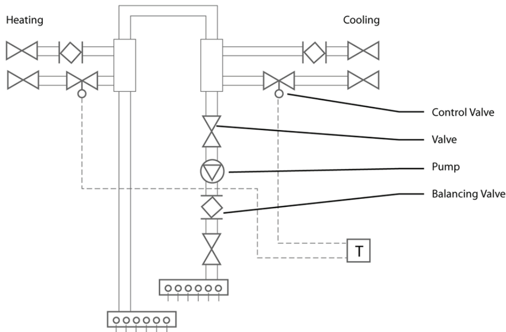
Figure A.1 — A typical radiant floor header connection
