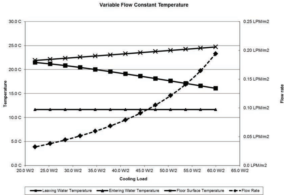
Figure A.3 — Variable flow constant supply water temperature control strategy
