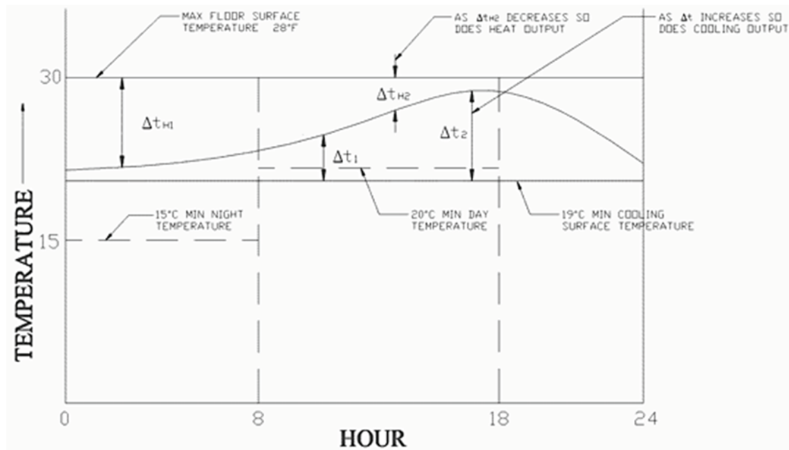
Figure 2 — Self-regulating effect of a radiant floor
