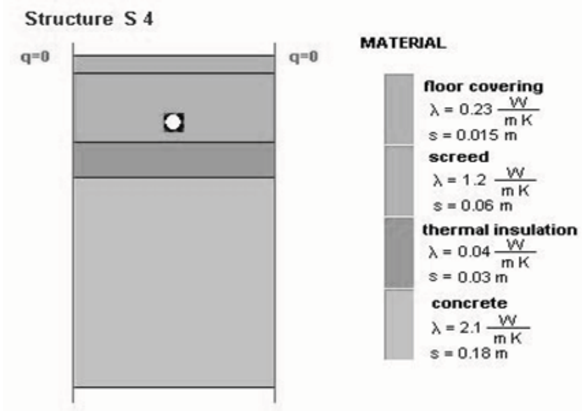
Figure D.1 — System construction and material properties for the test example
