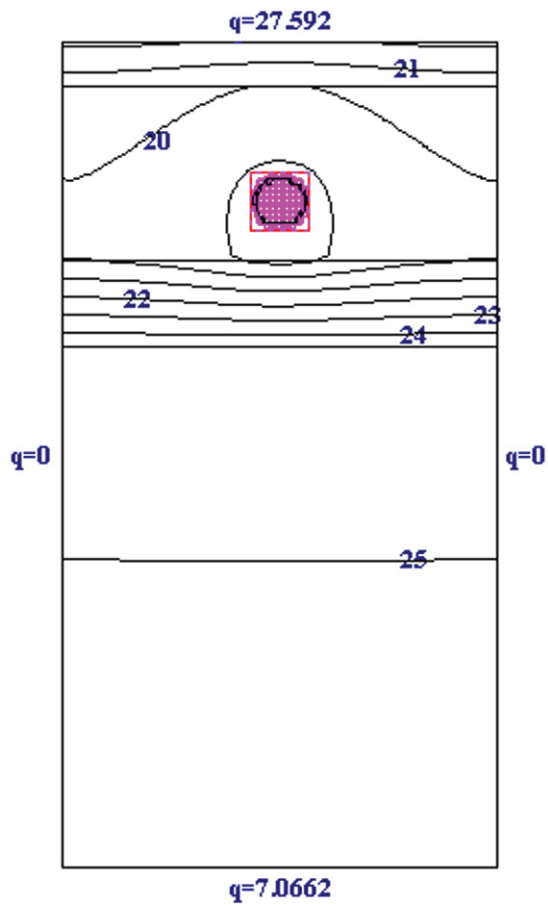
Figure D.2 — Results of temperature distribution
