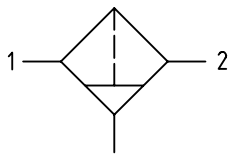
Filter
