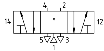
5/3 optional dual pressure valve
