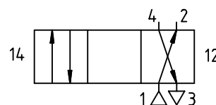
4/3 valve
