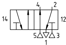
5/2 optional dual pressure valve
