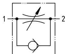
Flow control valve
