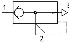
Lockout valve
