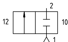
3/2 NO valve
