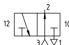
3/2 selector valve
