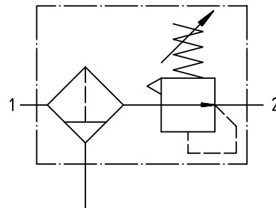
Filter-regulator
