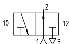
3/2 diverter valve
