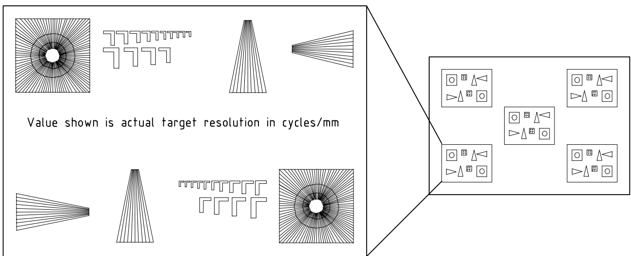
Figure 2 — Sample layout of test image type 2 for checking resolving power
