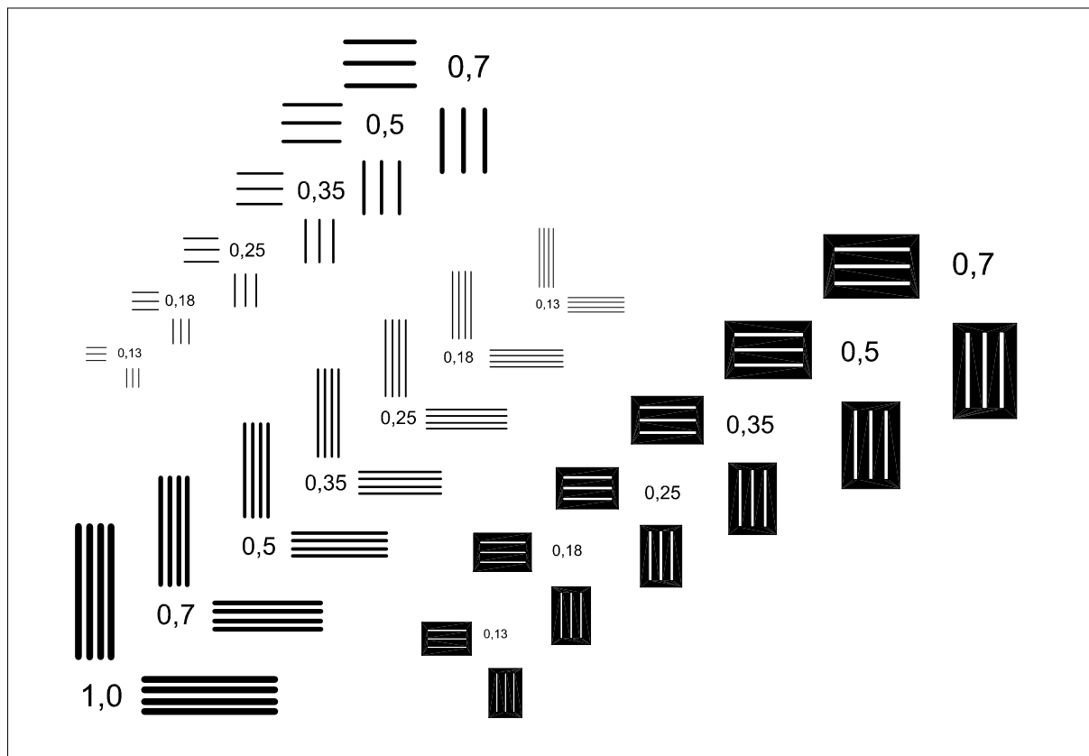
Figure 3 — Sample layout of test image type 3 (set of 5) for checking line width
