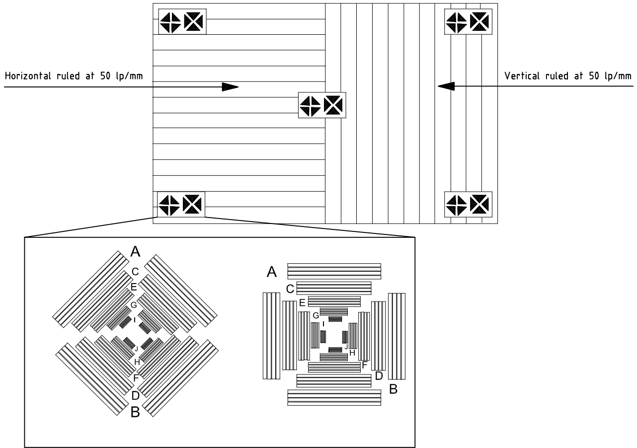
Enlarged detail of test target
