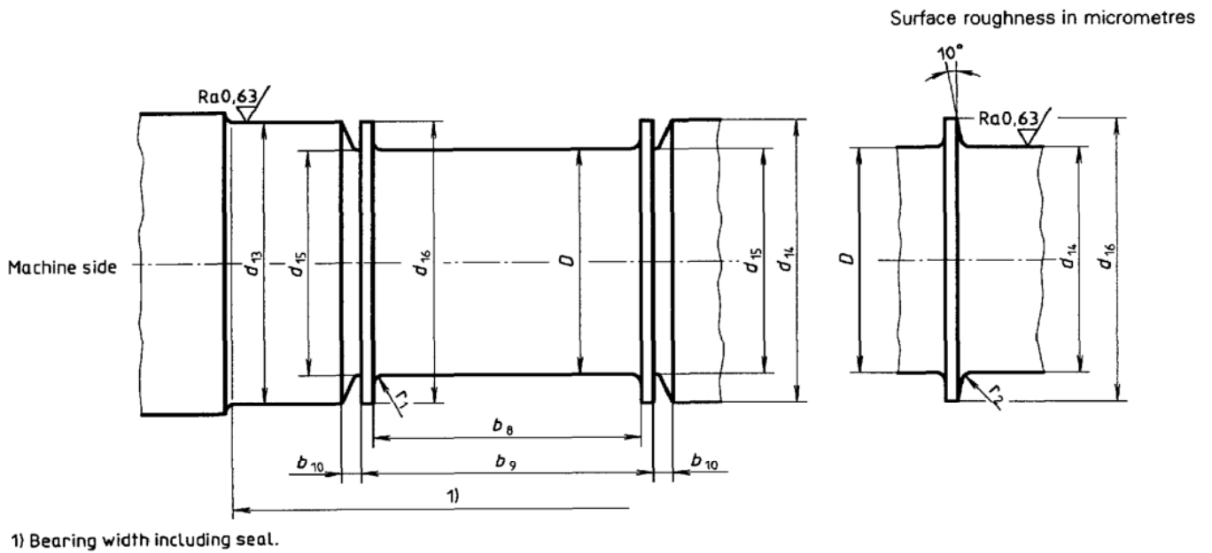
Figure 2 — Shaft design for non-locating (free) bearing (thrust bearing part Q)
