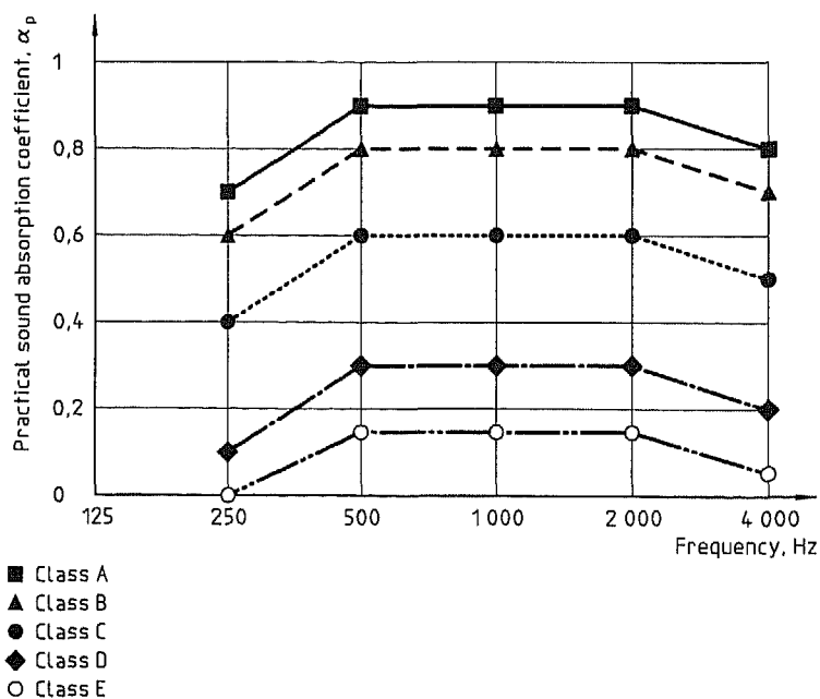
Figure B.1 — Illustration of the reference curves limiting the different sound absorption classes
