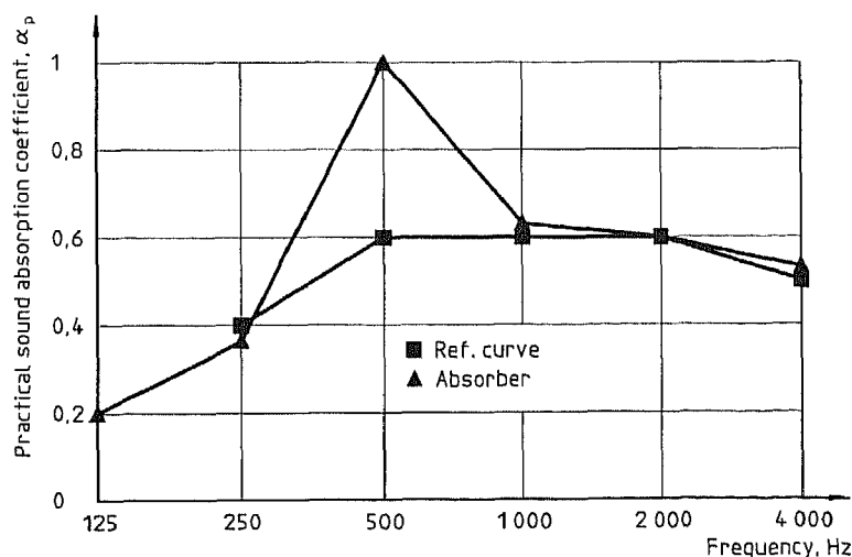
Figure A.2 — Example of a calculation of \alpha_w [ \alpha_w = 0,60(M) ]
