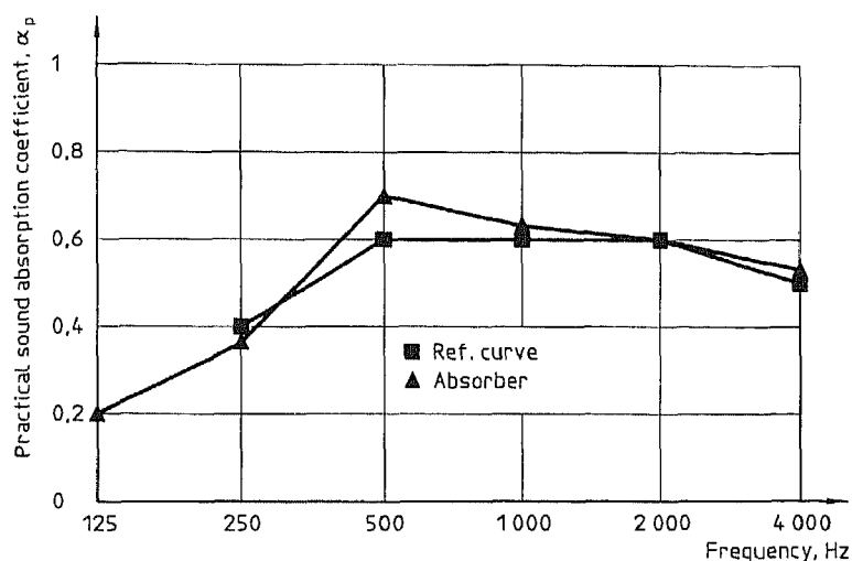
Figure A.1 — Example of a calculation of \alpha_w ( \alpha_w = 0,60 )
