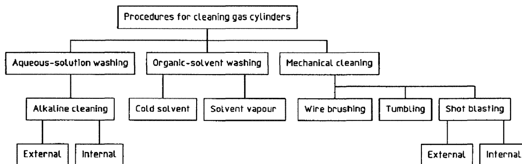
Figure A.1 — Methods used to clean gas cylinders
