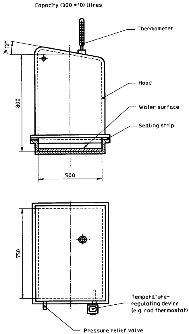
Figure 2 — Airtight cabinet with hood
