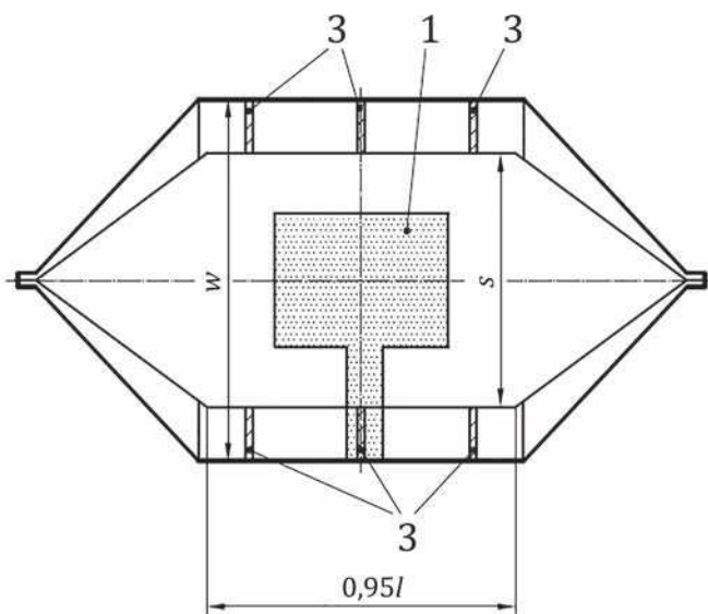
a) Horizontal section view through septum
