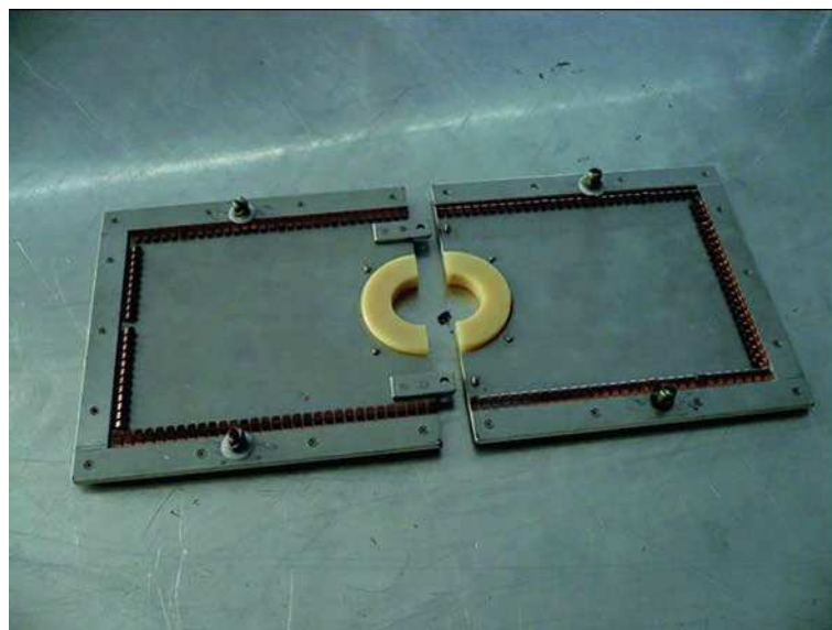
Figure D.3 — Example of through-hole panel
