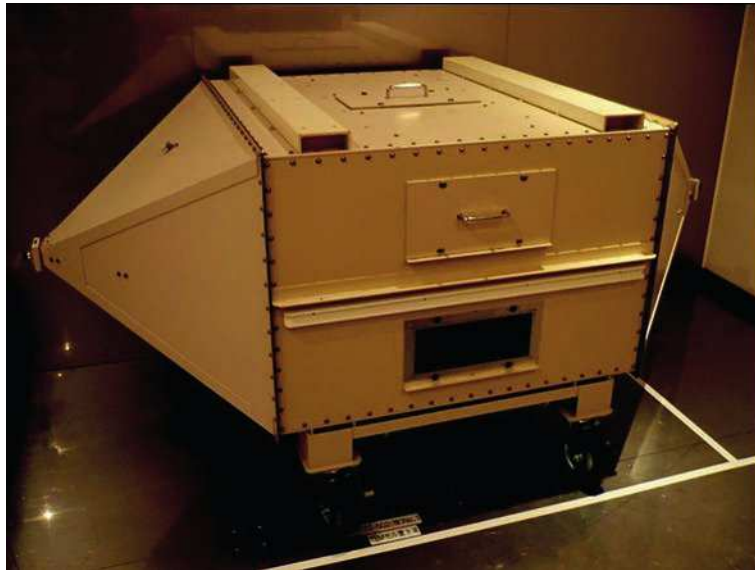
Figure D.4 — Example of TEM cell before attaching a through-hole panel
