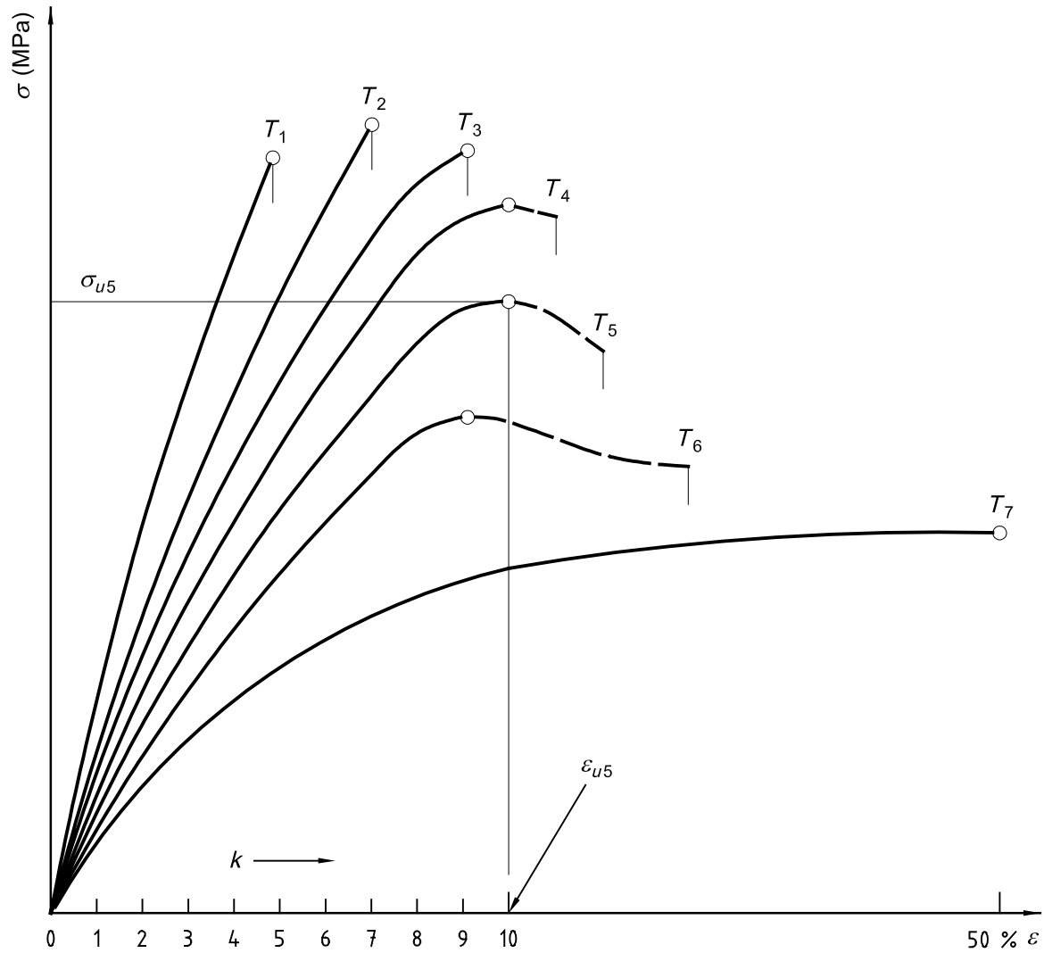
Figure 2 — Stress-strain curves at different temperatures T_i showing ultimate values of stress \sigma_{U_i} and strain \epsilon_{U_i} and identifying strains \epsilon_{k_i} = \epsilon_{U_i} \times k/10 at which values of stress are to be recorded
