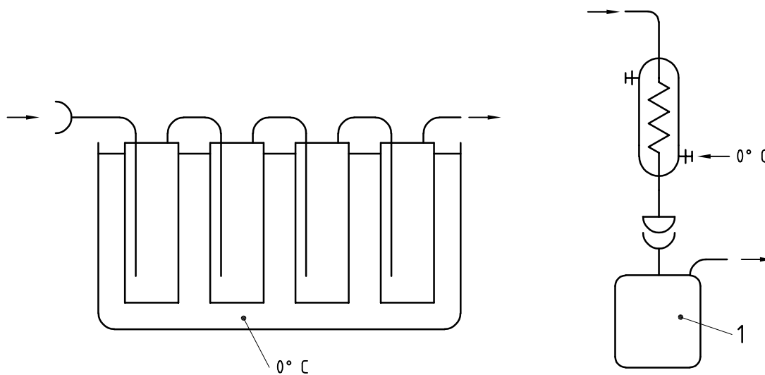
Figure B.4 — Two types of particle filter
