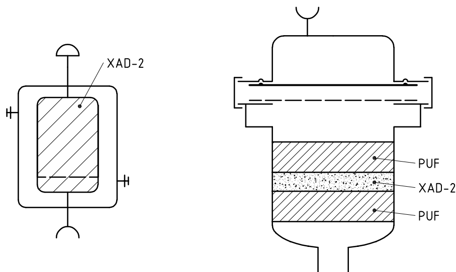
Figure B.6 — Two types of adsorber cartridge
