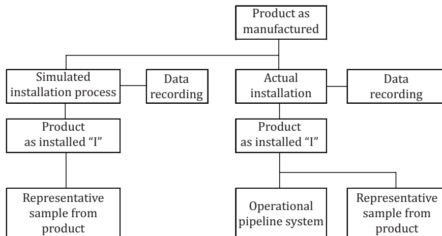
Figure 3 — Relationship between samples taken from simulated and actual installations
