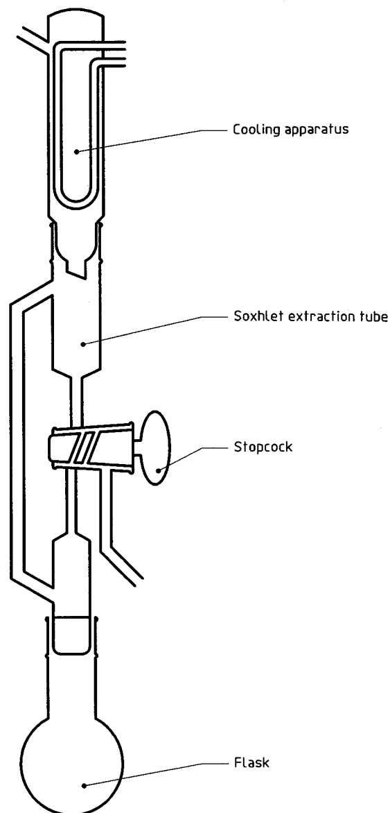
Figure 1 — Digestion apparatus
