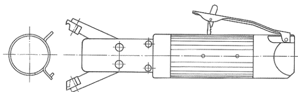
Figure B.4 — Crimping pliers
