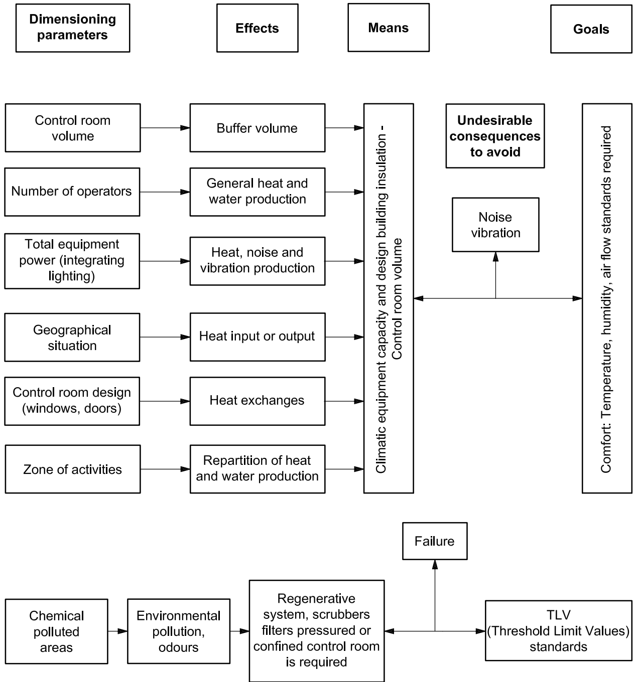
Figure 2 — Main factors in design of thermal environments, air quality and acoustic parameters
