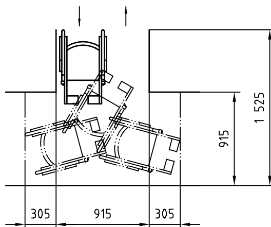
b) Minimum dimensions for T-shaped turning space
