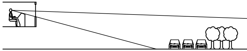
Figure A.1 — Recommended view out with direct view of sky reduced
