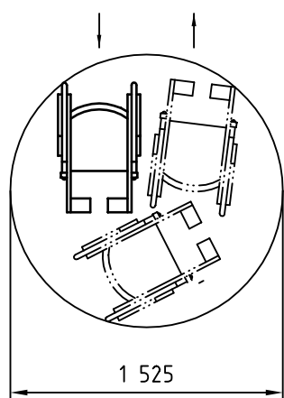
a) Minimum diameter for circular turning space
