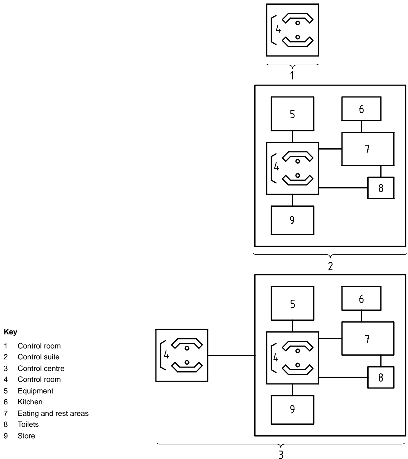
Figure 1 — Schematic illustrations of control room, control suite and control centre
