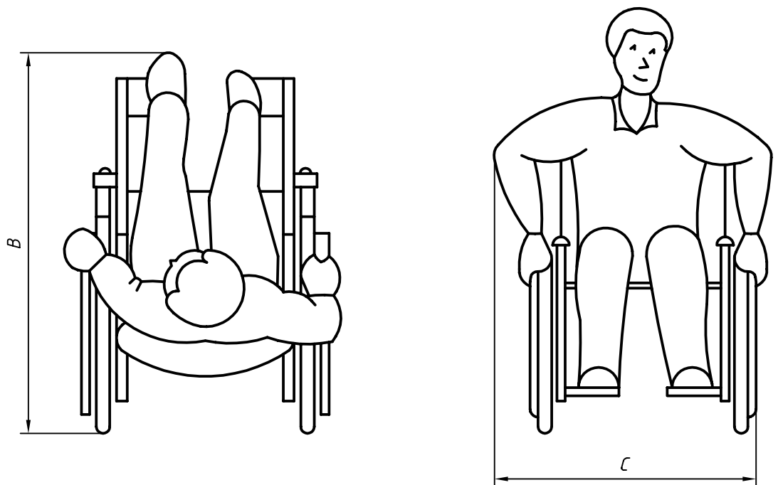
Figure 9 — Wheelchair clearance
