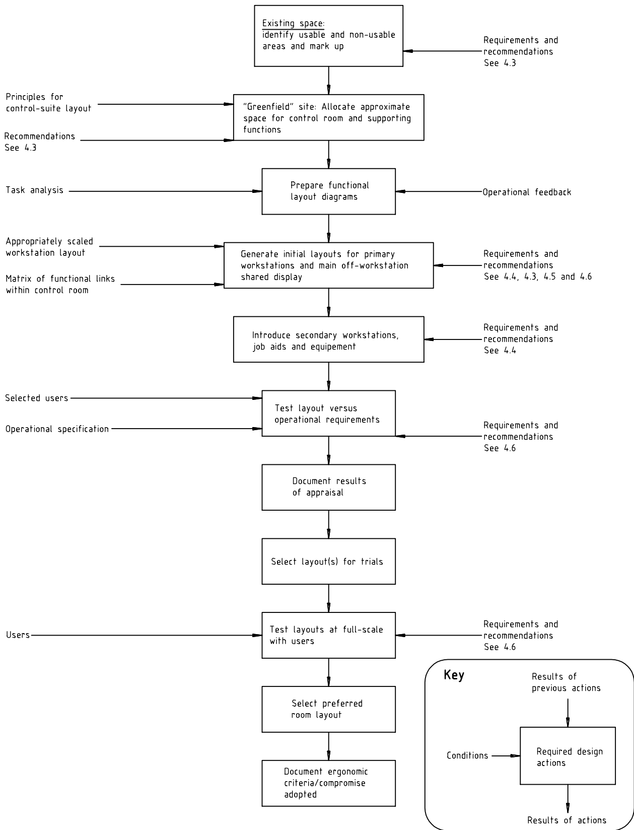
Figure 3 — General procedure for control room layout
