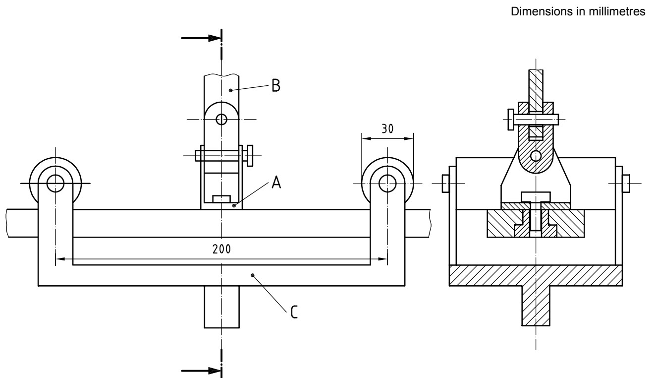
Figure 2 — Universal test machine with pull-out device
