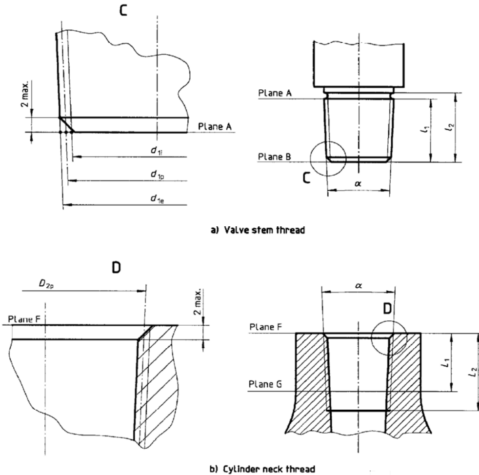
Figure 1 — Thread reference planes and diameters
