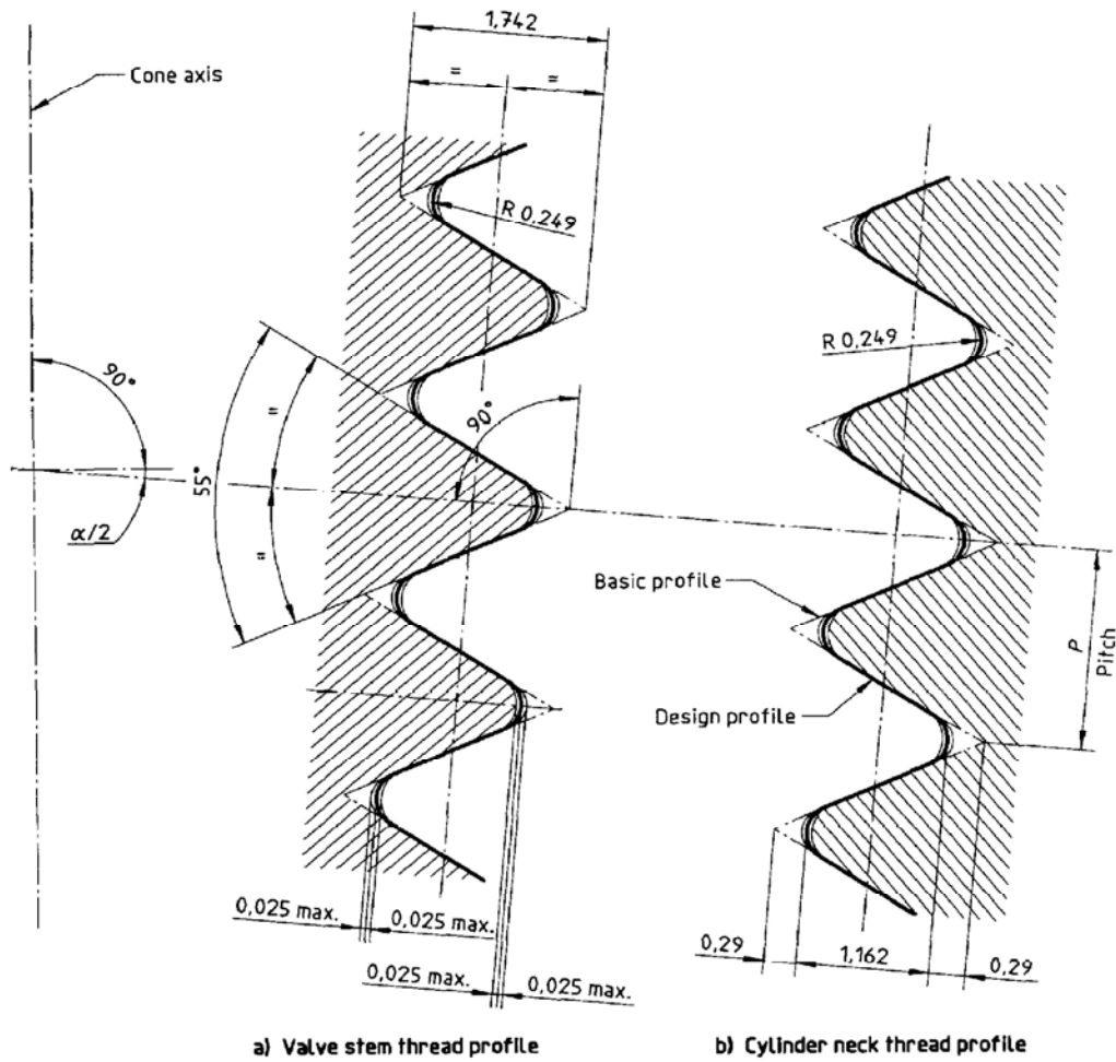
Figure 2 — Thread profiles
