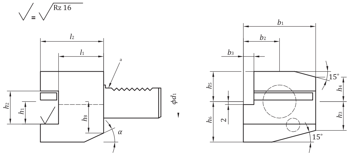
Figure 1 — Type B1 tool holder, right-hand, short
