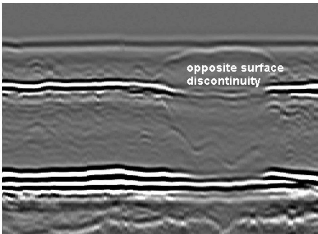
Figure B.11 — Elongated TOFD indication of a far-surface-breaking discontinuity (nearly through-wall)
