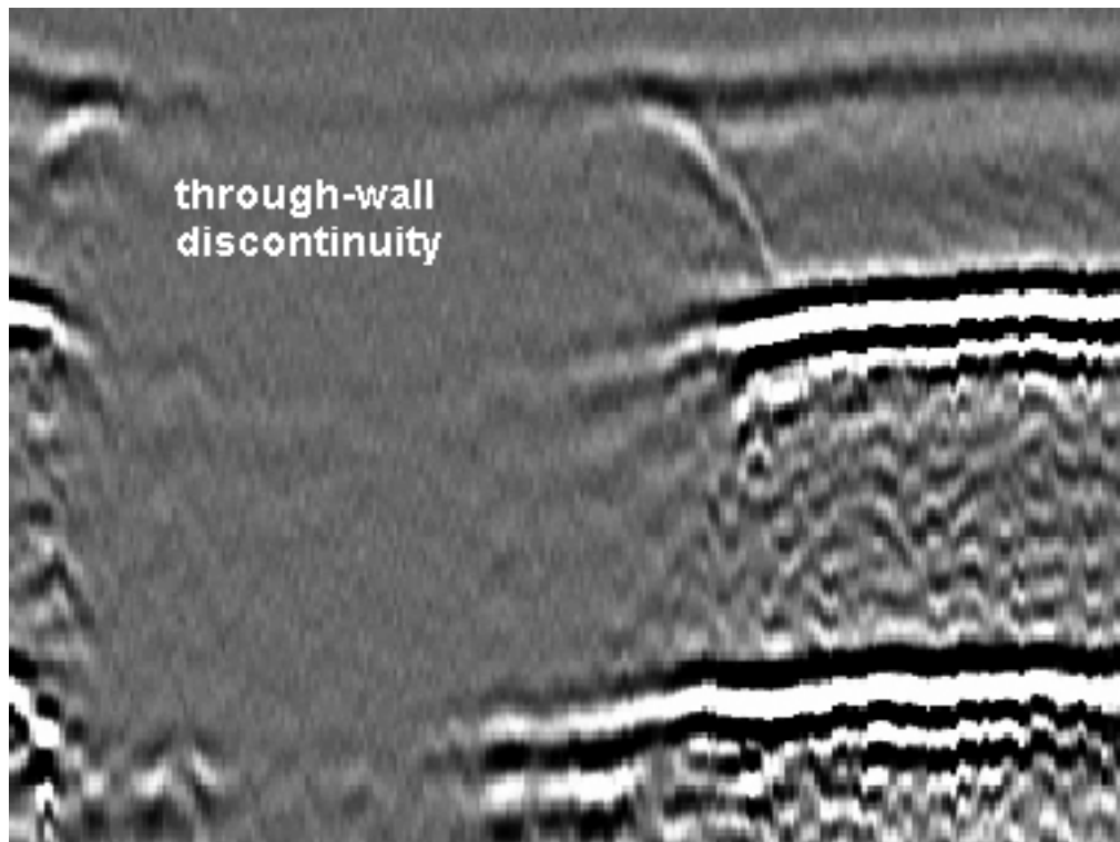
Figure B.12 — TOFD indication of through-wall crack (note the loss of lateral wave and back-wall signal and also the corresponding diffracted signal patterns left and right of this region)
