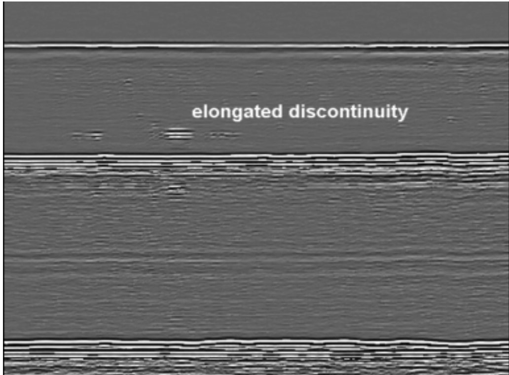
Figure B.14 — TOFD indication of an elongated discontinuity with measurable height
