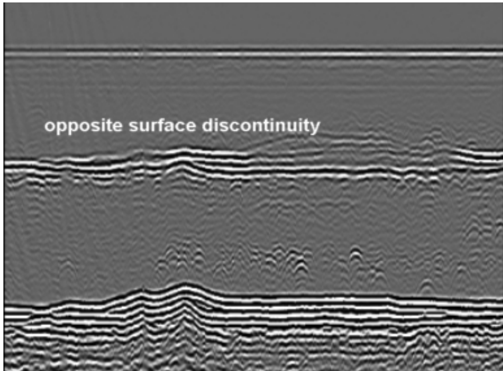
Figure B.10 — Elongated TOFD indication of an opposite surface-breaking discontinuity
