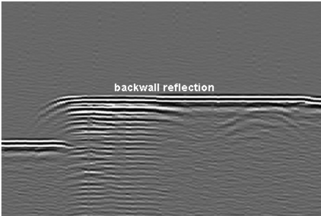
Figure B.15 — TOFD indication of change in wall thickness
