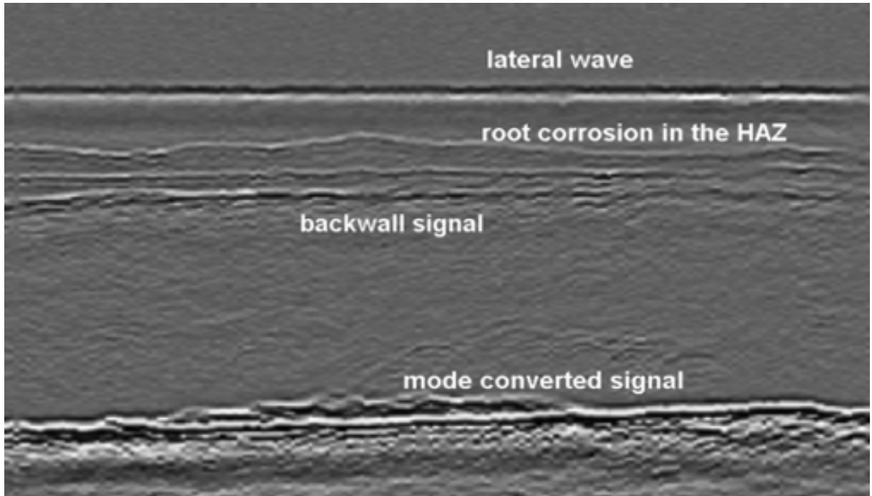
Figure B.18 — TOFD indication of corrosion in the root area on both sides of the weld in the heat-affected zone
