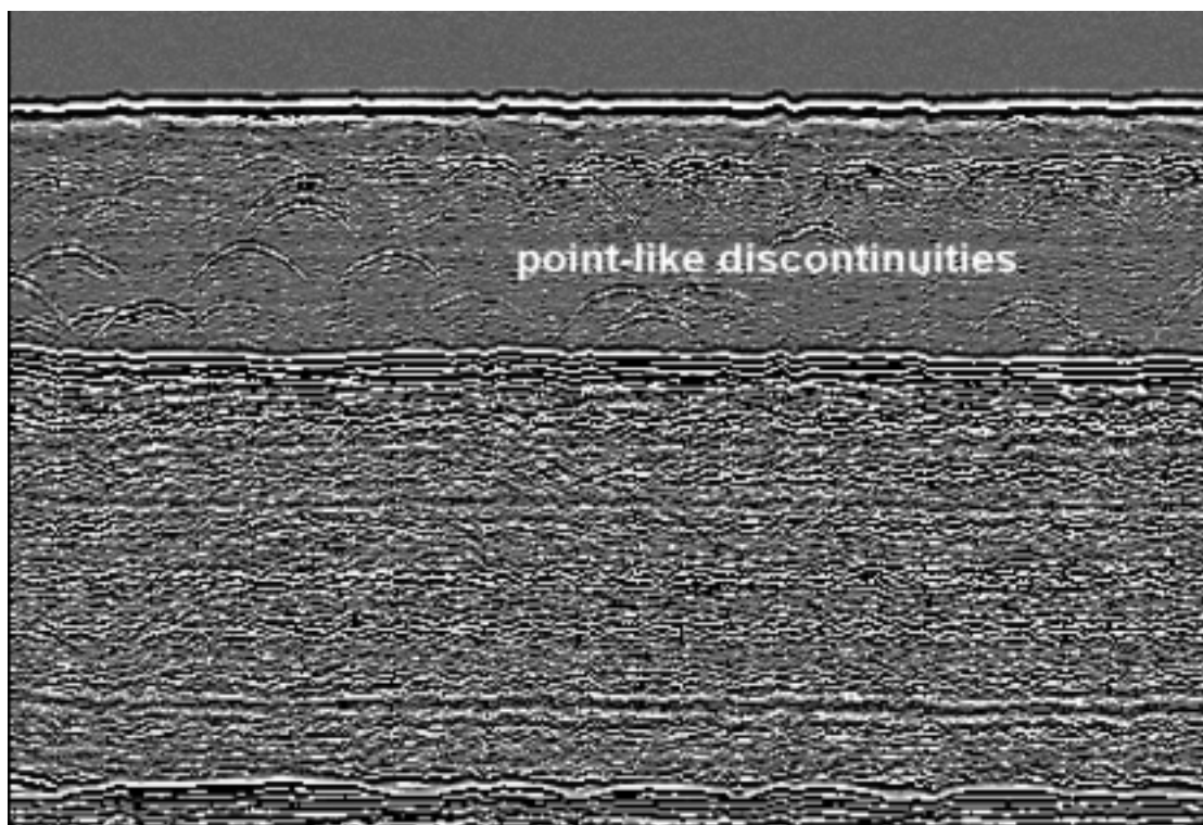
Figure B.13 — TOFD indications of multiple point-like discontinuities
