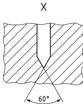
Figure A.3 — Detail of notch tip
