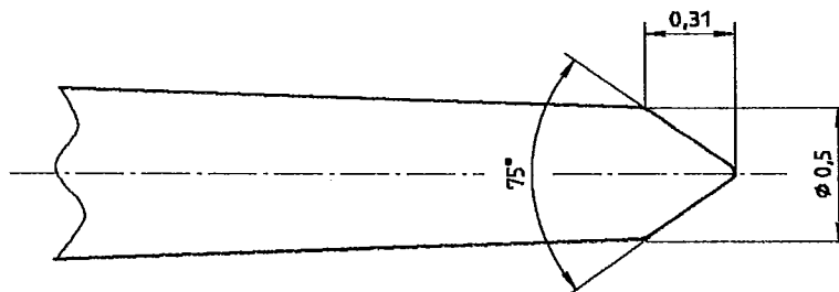
Figure 2 — Tip of a tapestry needle
