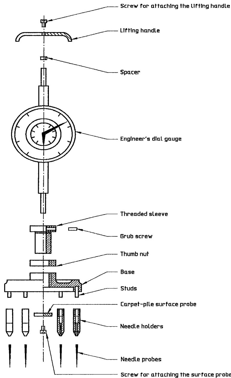
Figure 1 — Exploded diagram of the WRONZ pile-thickness gauge
