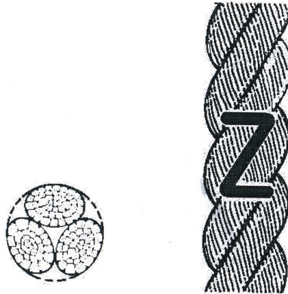
Figure 1 — Shape of a 3-strand hawser-laid rope (type A)
