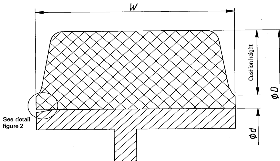
Figure 1 — Cylindrical base solid tyre
