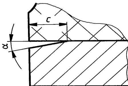
Figure 2 — Rim beveling
