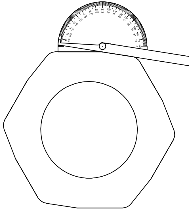
Figure 18 — Measurement of kelly wear-pattern angle
