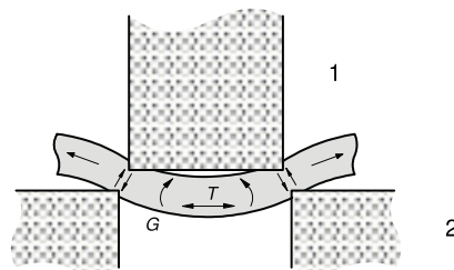
Figure 8 — Combinations of test pieces and test machine contact surfaces
