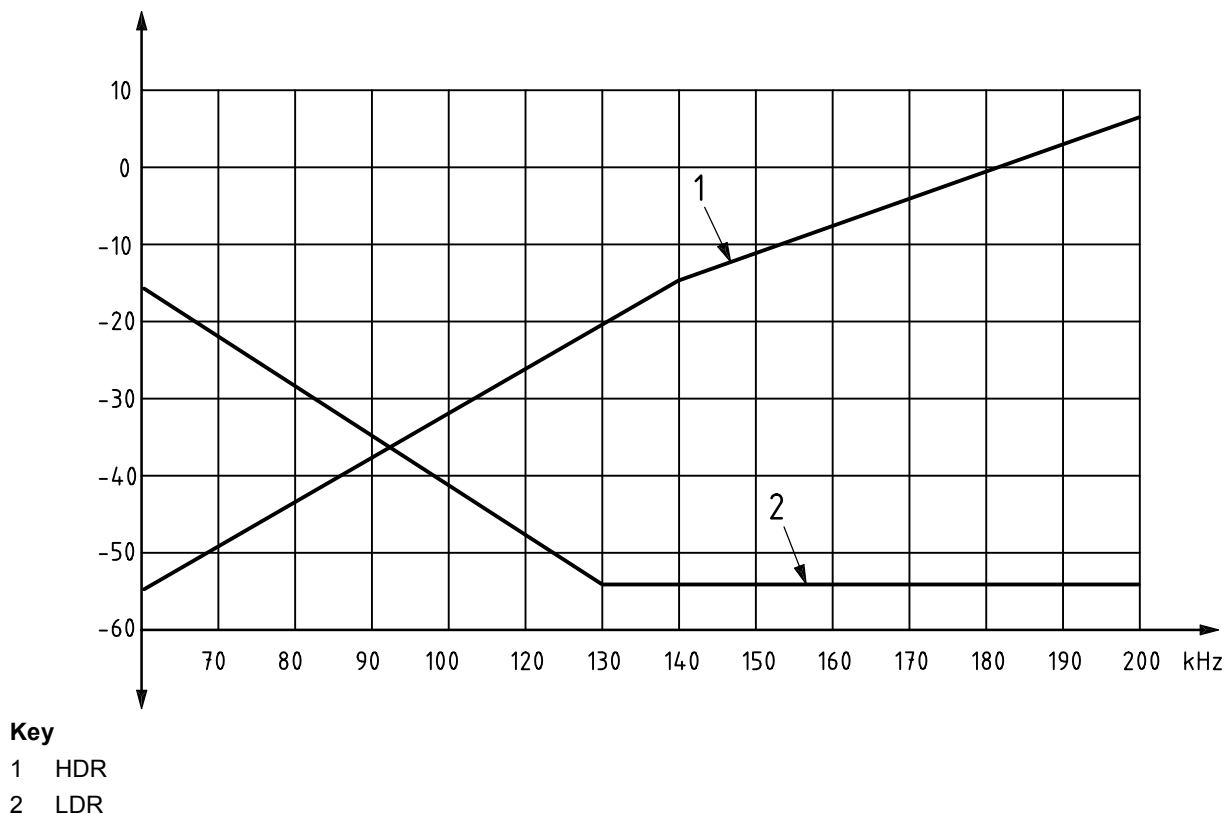
Figure 23 — Filter specifications — Low data rate compatibility
