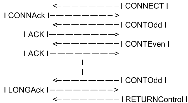
Figure 17 — RCD device poll session transfer diagram
