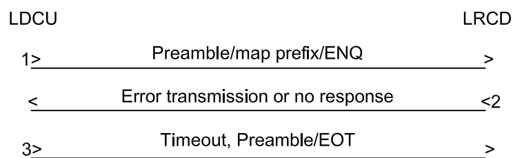
Figure 14 — Unidentified map session transfer diagram
