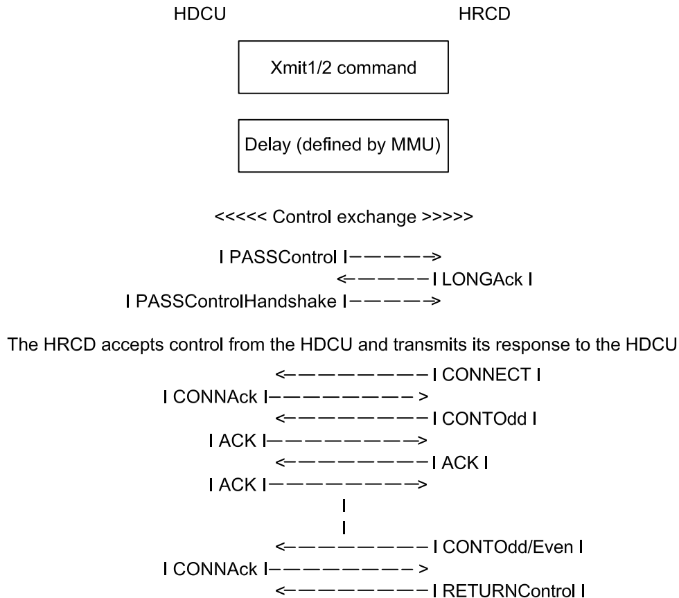
Figure 19 — RCD/device interactive1/2 session transfer diagram
