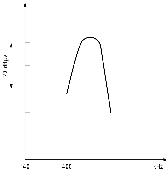
Figure 22 — Power density function
