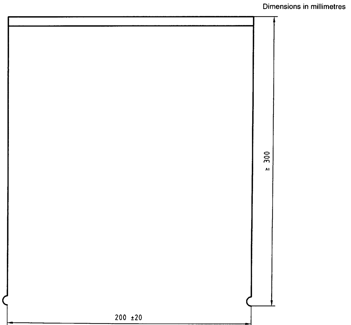
Figure 4 — Test yoke
