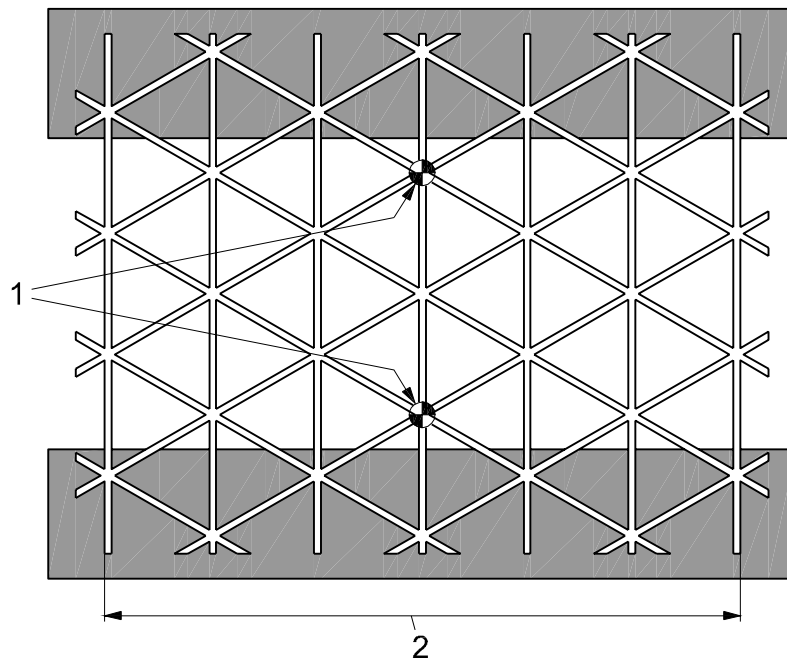
Figure 6 — Example of geogrid with three axes, specimen size, widths and gauge length MD
