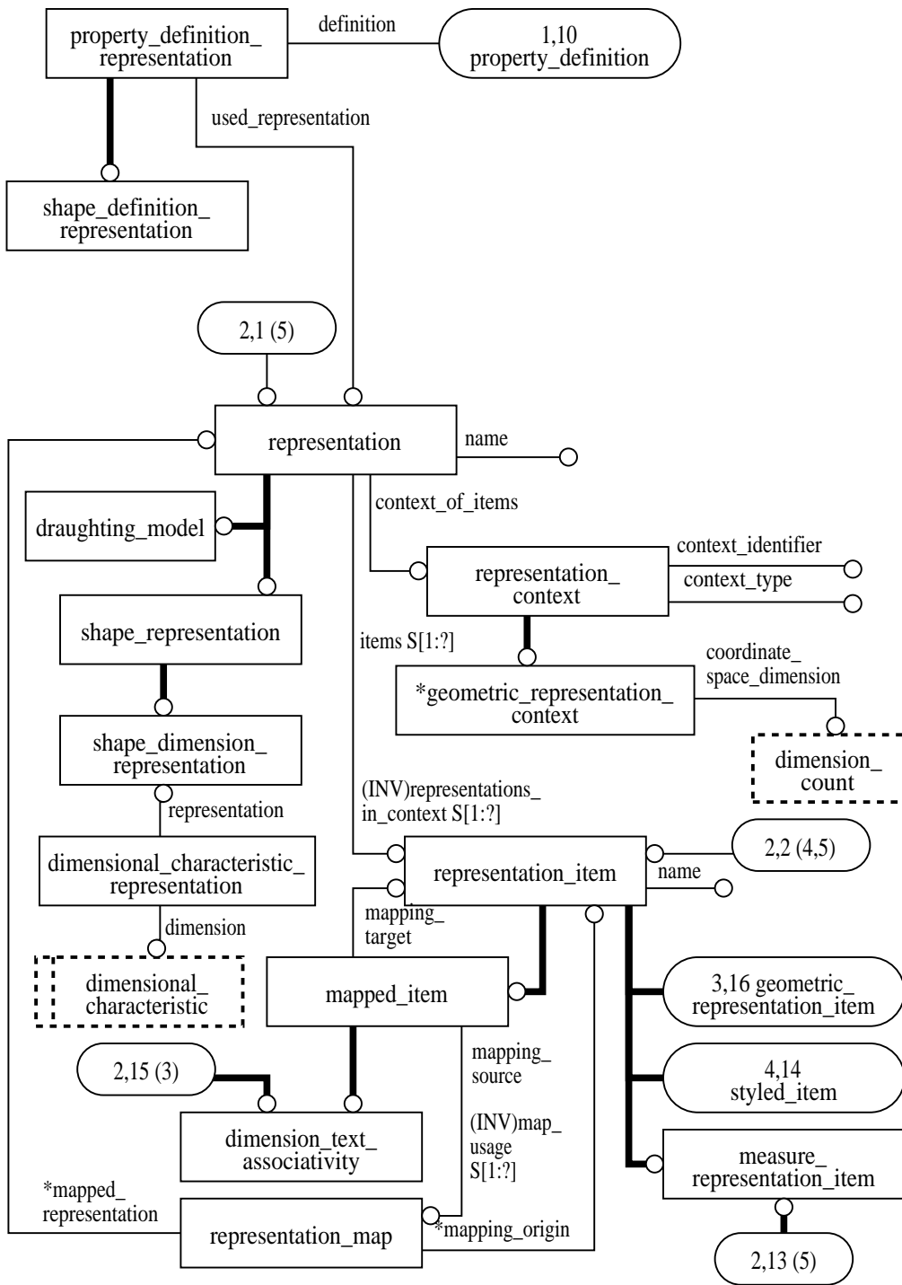
Figure C.2 – AIC expanded listing diagram in EXPRESS-G: 2 of 6
