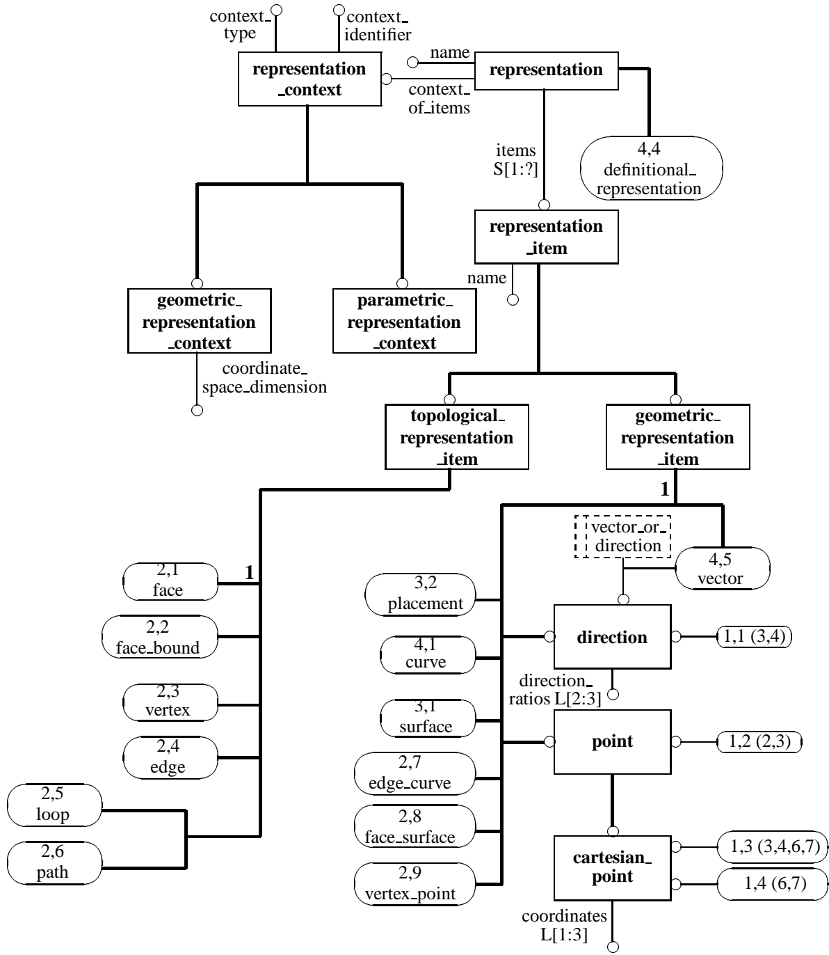
Figure D.1 – aic_topologically_bounded_surface EXPRESS-G diagram page 1 of 8
