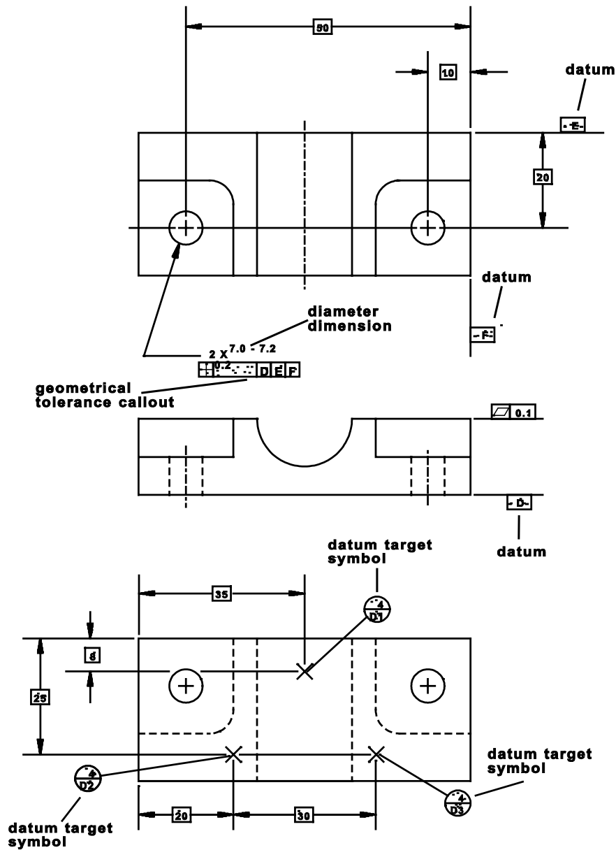
Figure 3 - Draughting callouts
