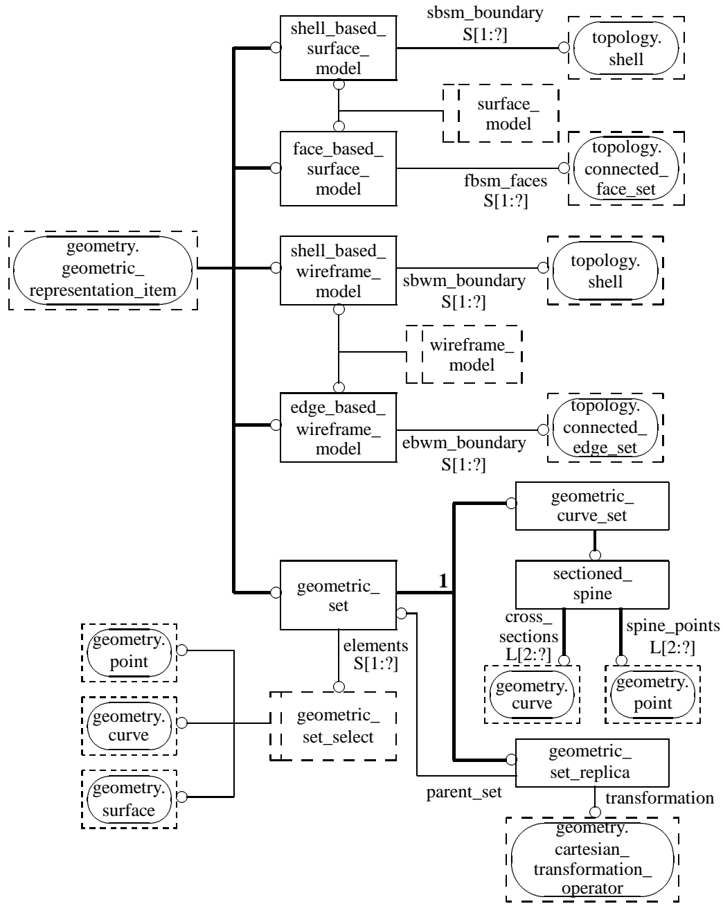
Figure D.19 – Geometric_model_schema EXPRESS-G diagram 3 of 4
