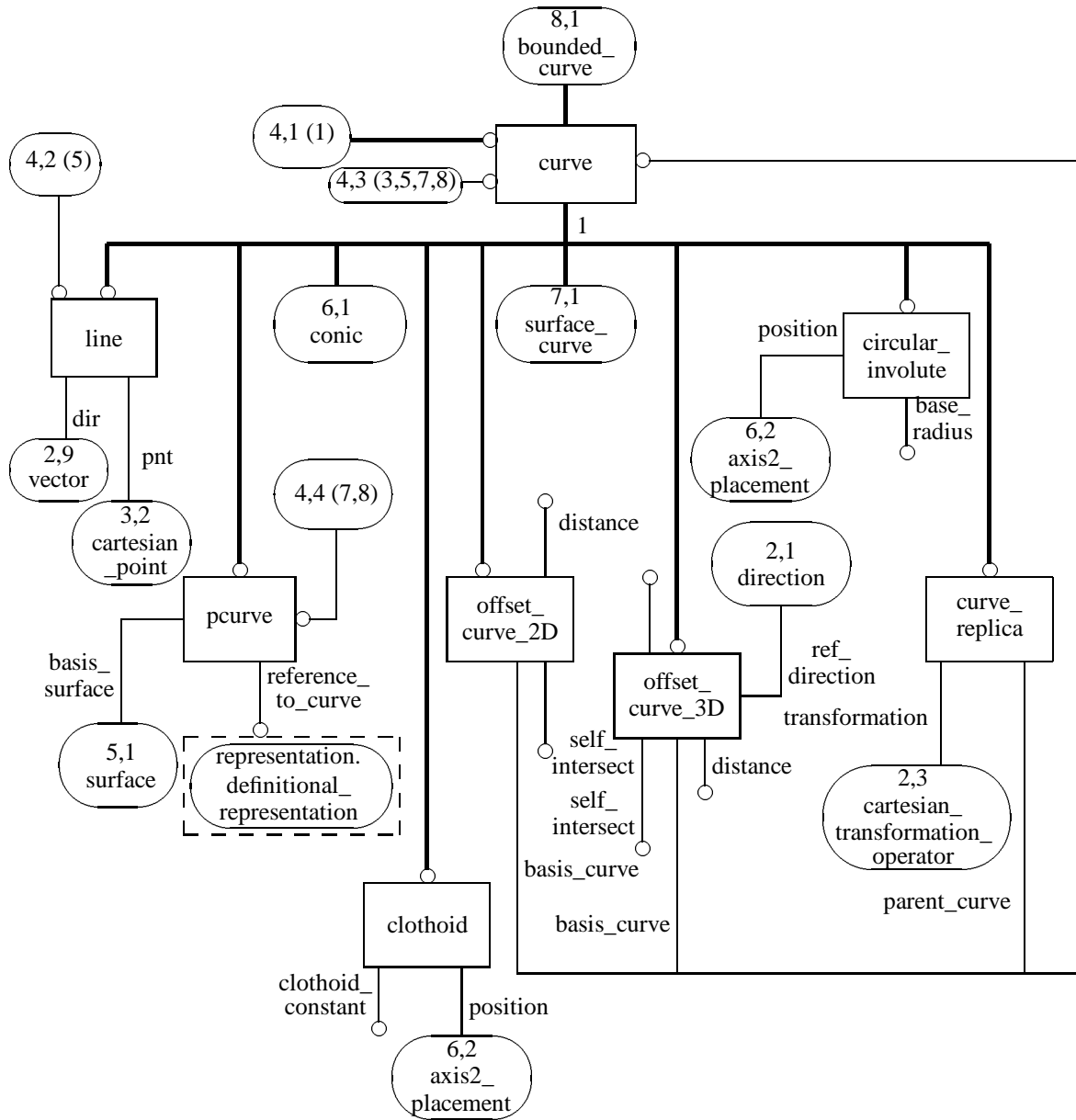
Figure D.4 – Geometry_schema EXPRESS-G diagram 4 of 13
