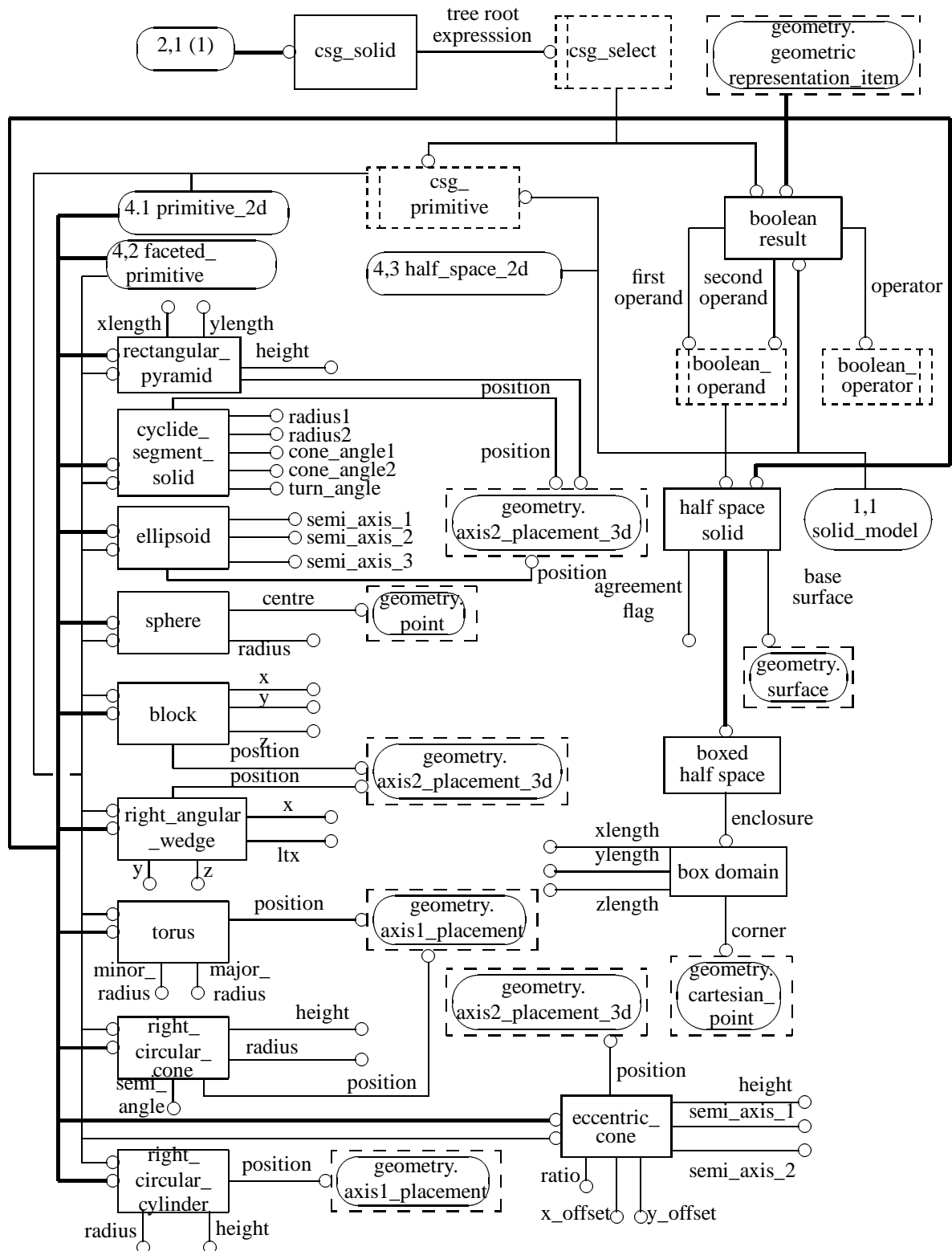
Figure D.18 – Geometric_model_schema EXPRESS-G diagram 2 of 4
