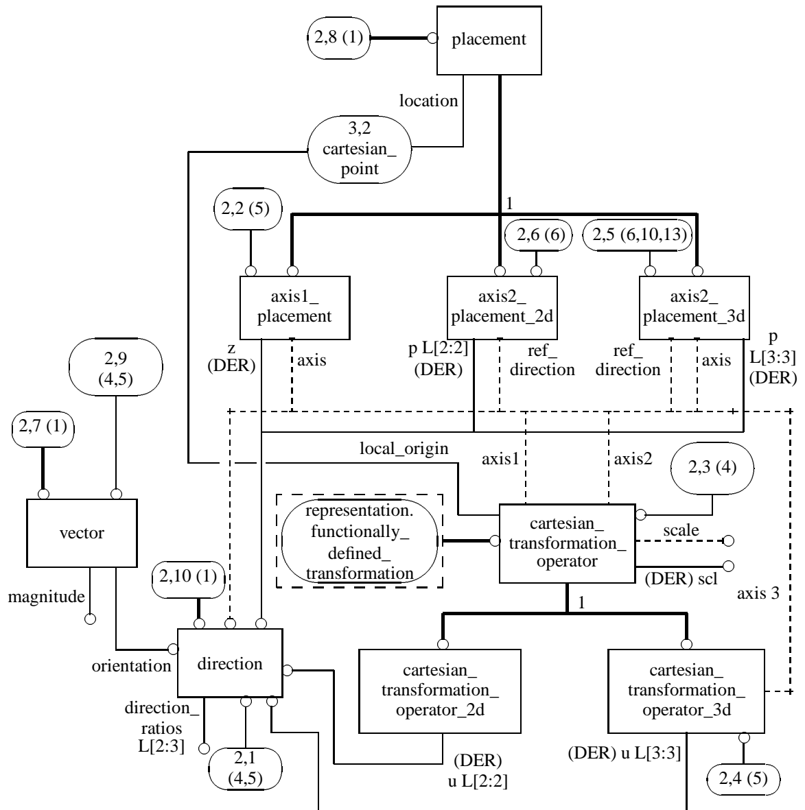
Figure D.2 – Geometry_schema EXPRESS-G diagram 2 of 13
