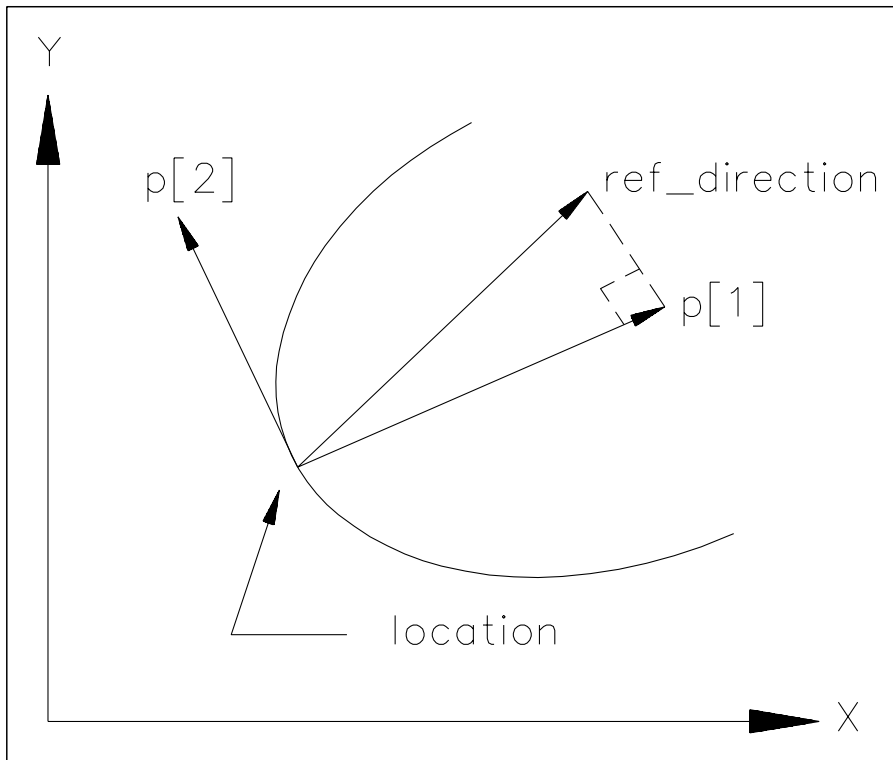
Figure 7 – Parabola
