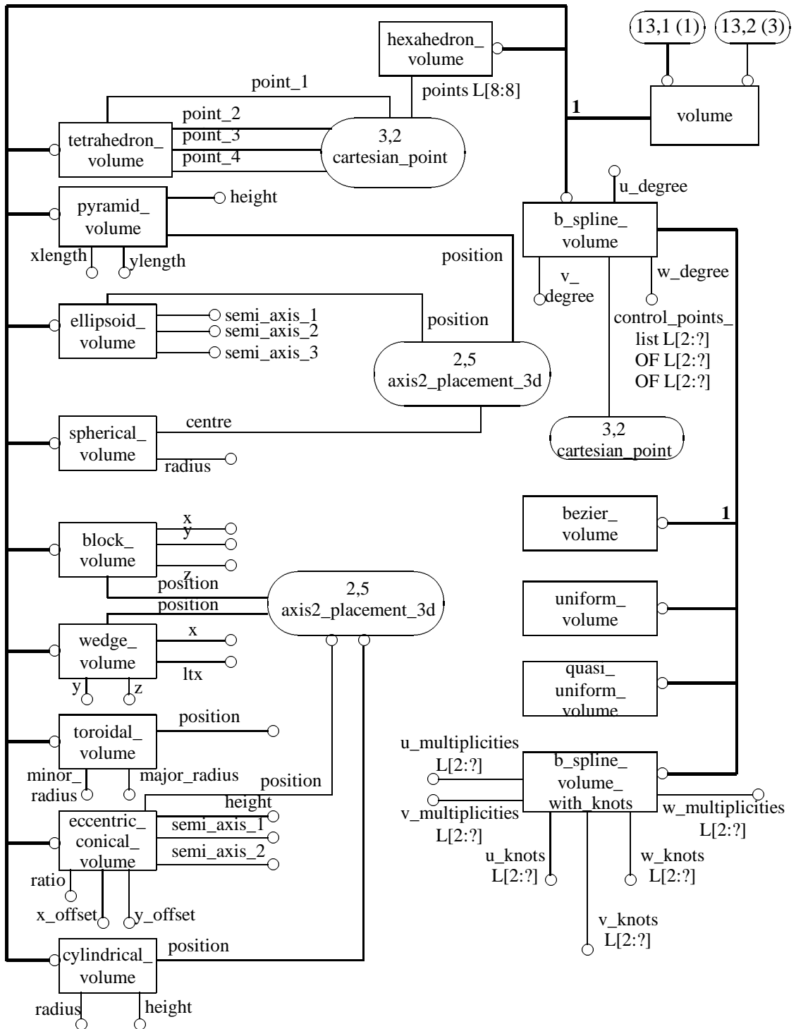
Figure D.13 – Geometry_schema EXPRESS-G diagram 13 of 13
