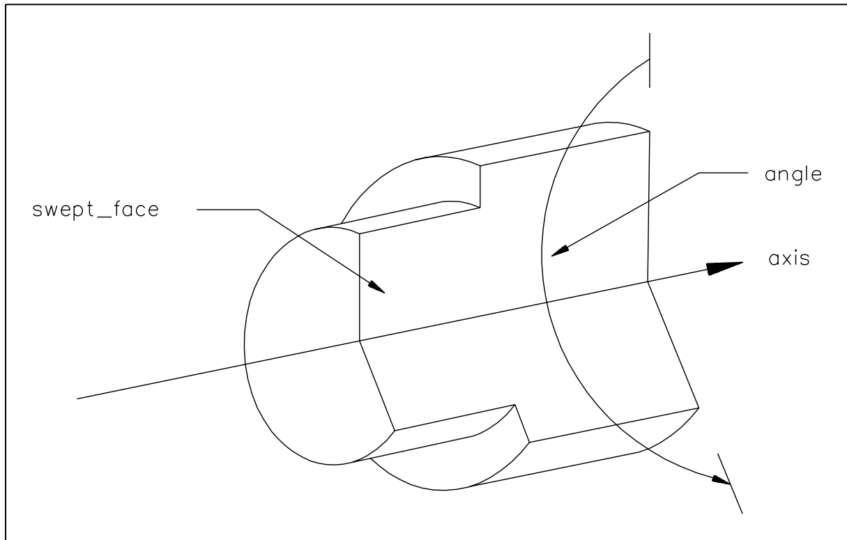
Figure 26 – Revolved face solid
