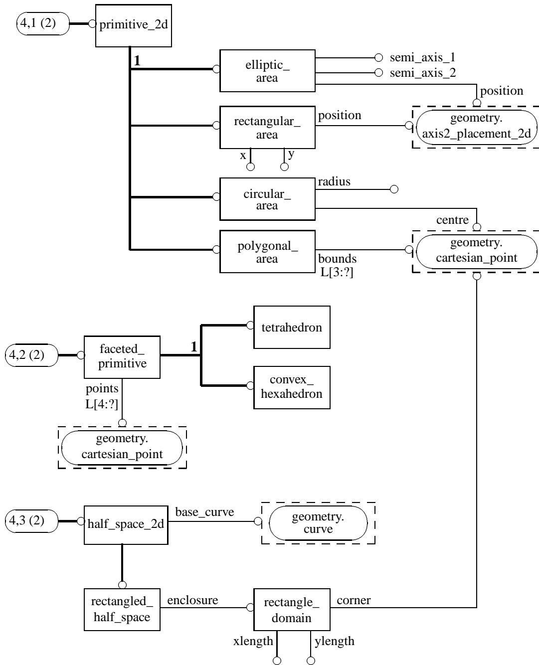
Figure D.20 – Geometric_model_schema EXPRESS-G diagram 4 of 4
