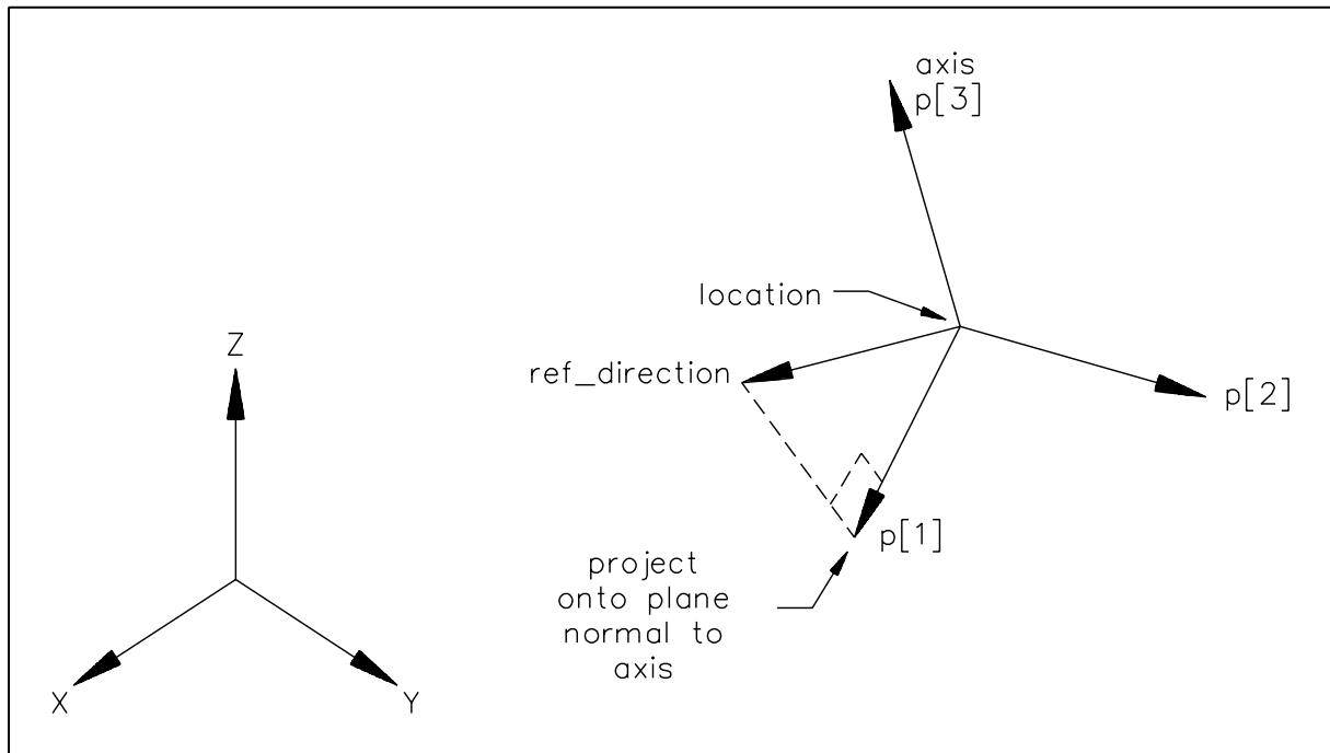
Figure 2 – Axis2_placement_3d
