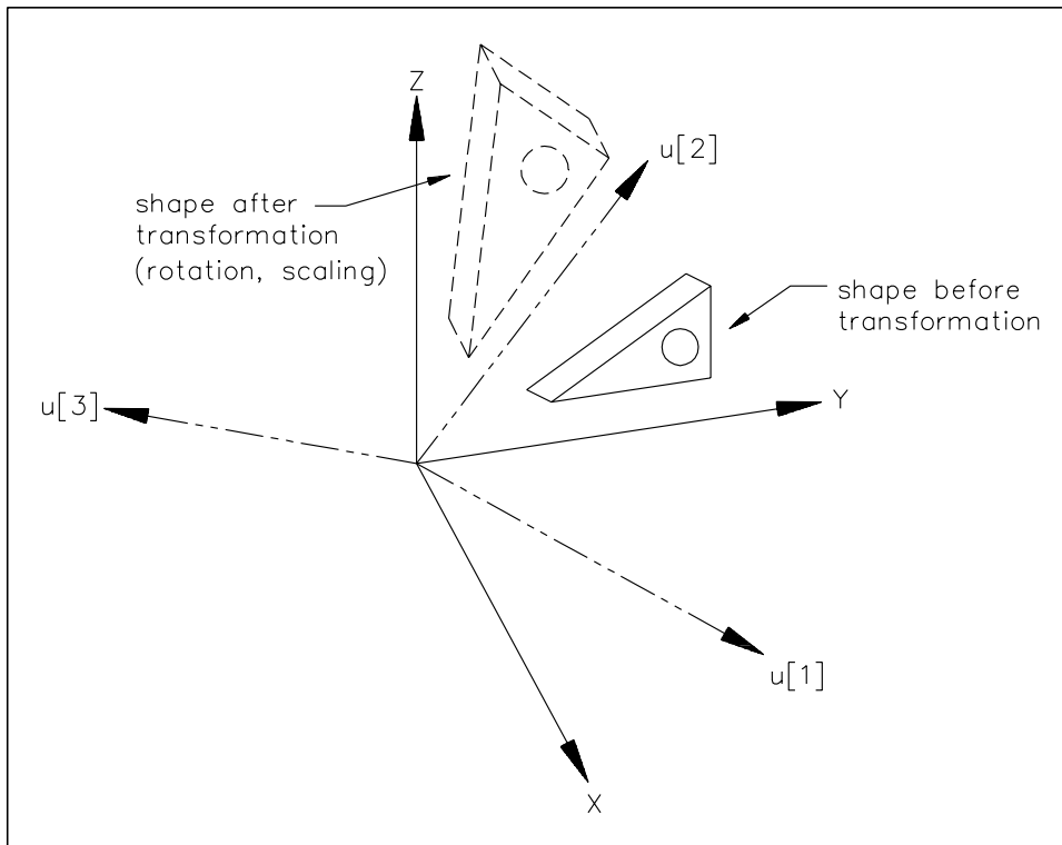
Figure 3 – (b) Cartesian_transformation_operator_3d
