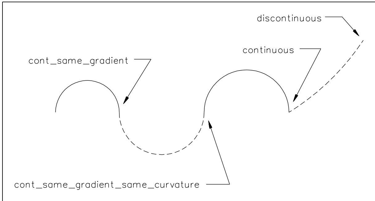
Figure 11 – Composite_curve
