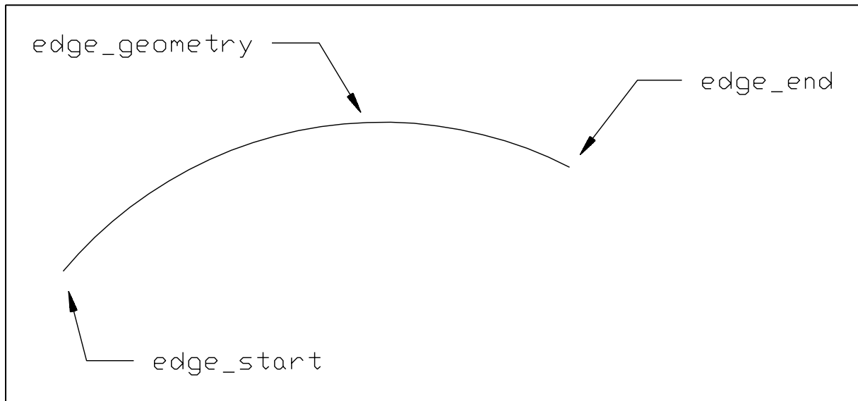
Figure 21 – Edge curve
