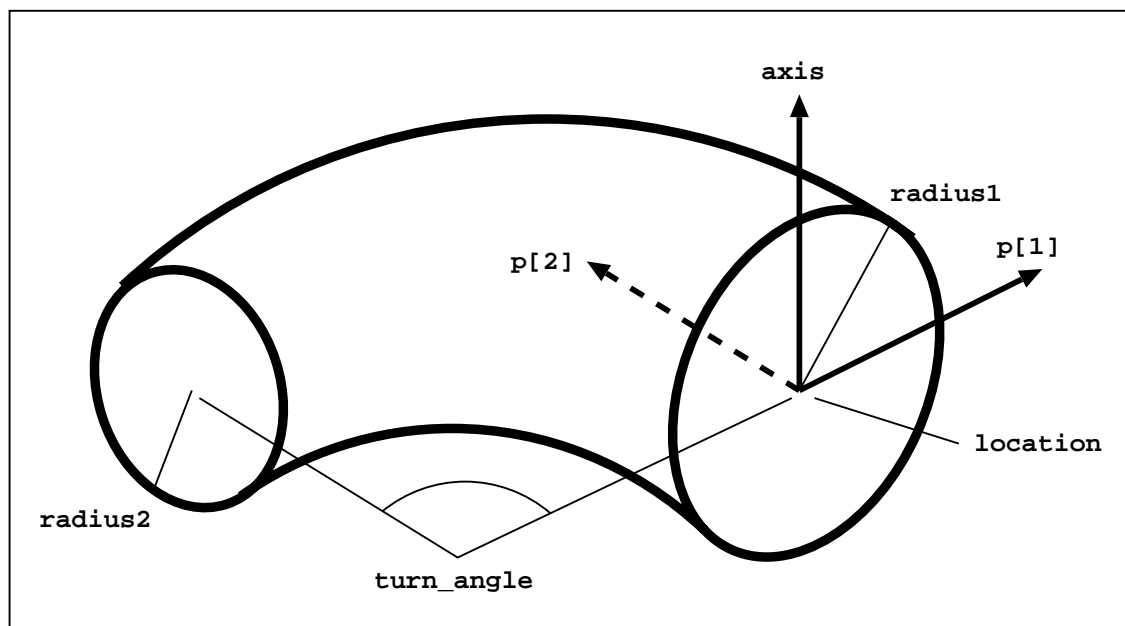
Figure 24 – Cyclide_segment_solid
