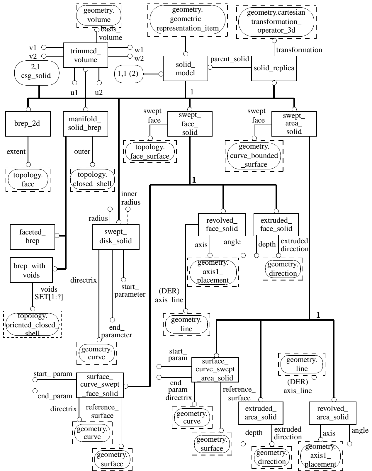
Figure D.17 – Geometric_model_schema EXPRESS-G diagram 1 of 4
