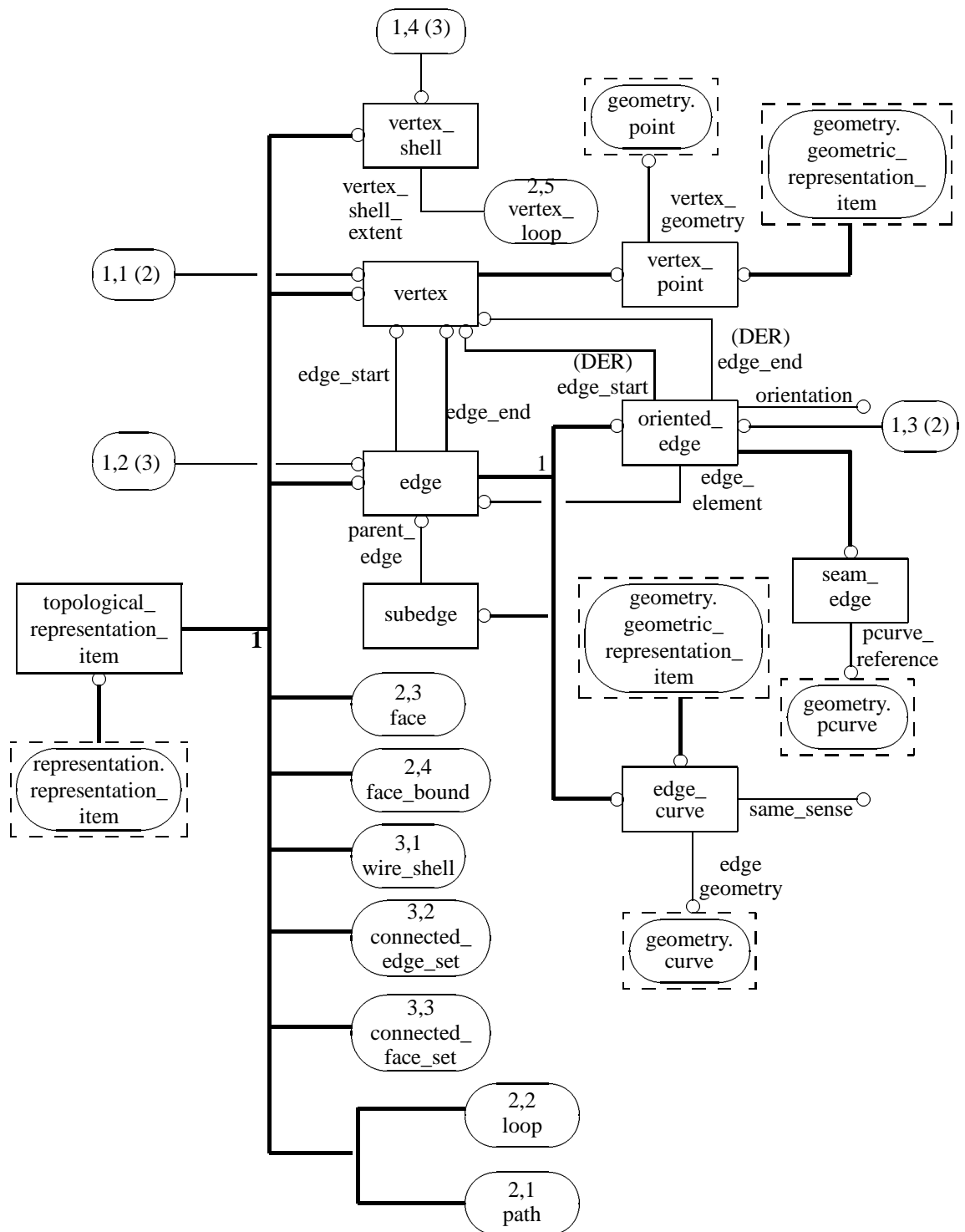
Figure D.14 – Topology_schema EXPRESS-G diagram 1 of 3
