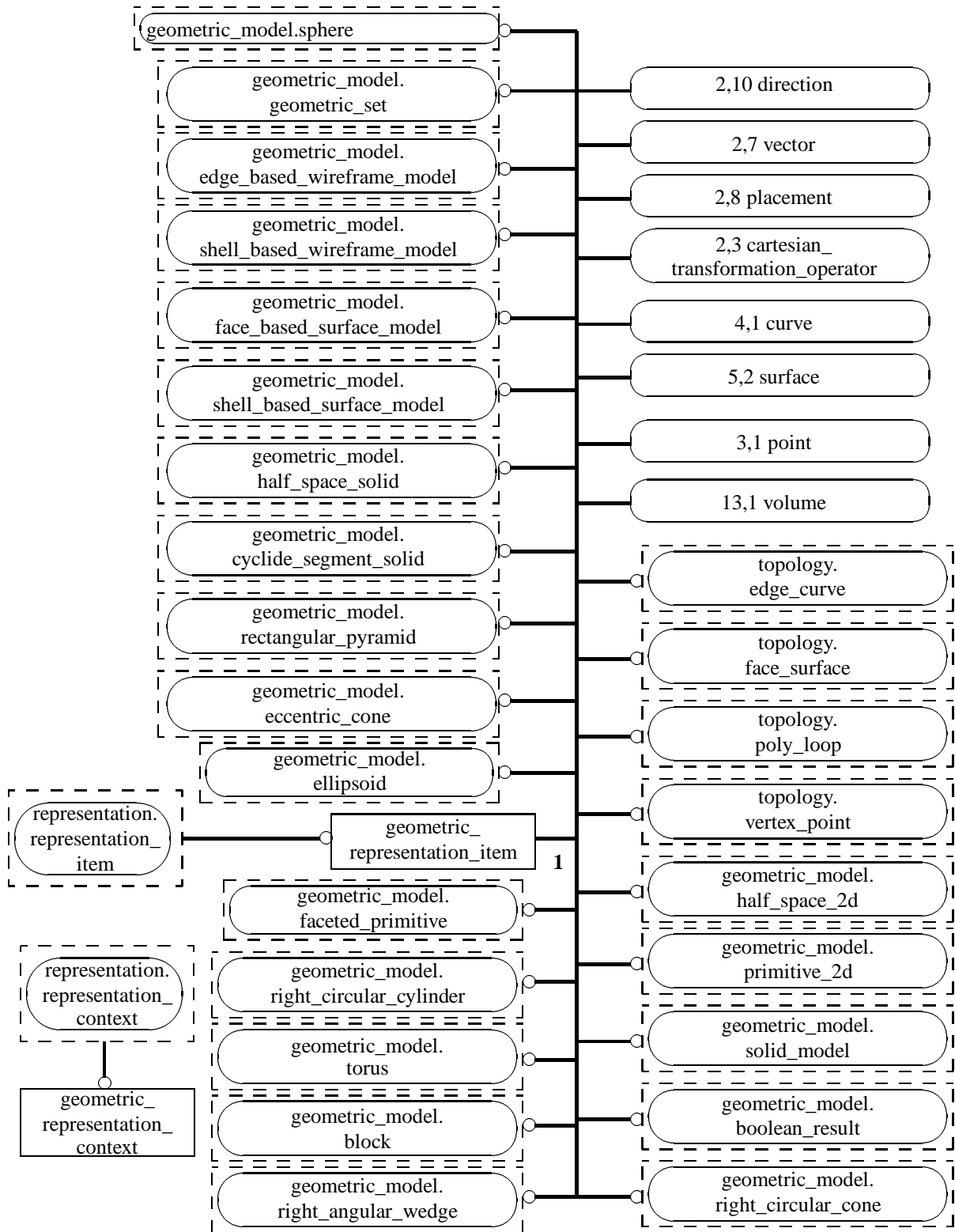
Figure D.1 – Geometry_schema EXPRESS-G diagram 1 of 13
