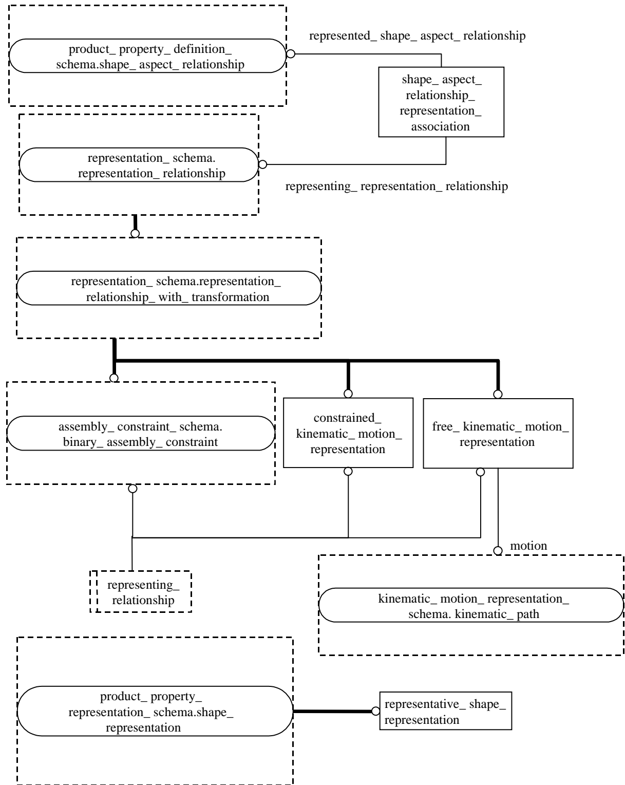
Figure D.1 – EXPRESS-G diagram of the assembly_feature_relationship_schema(1 of 1 )
