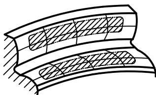
e) Slight lame pattern, still 80 % to 85 % coverage
