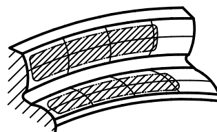
f) Slight toe pattern, still 80 % to 85 % coverage
