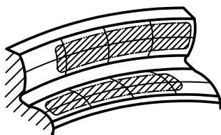
c) Slight cross pattern, still 80 % to 85 % coverage
