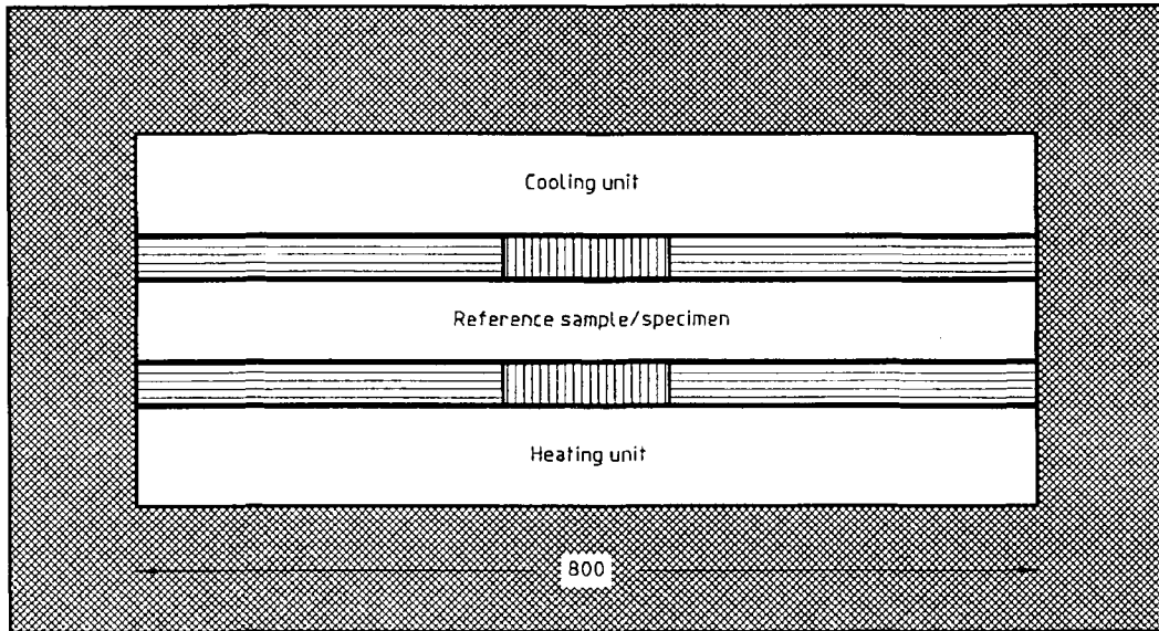
a) Single-specimen apparatus
