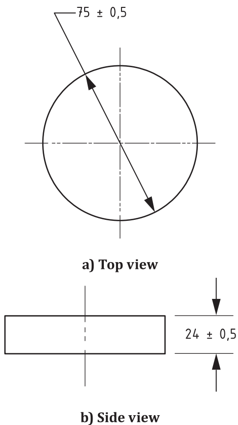
Figure 3 — Test disk (penetrator)
