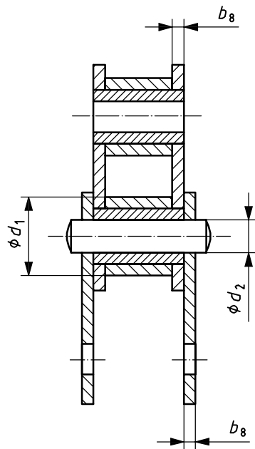
a) Roller chain
