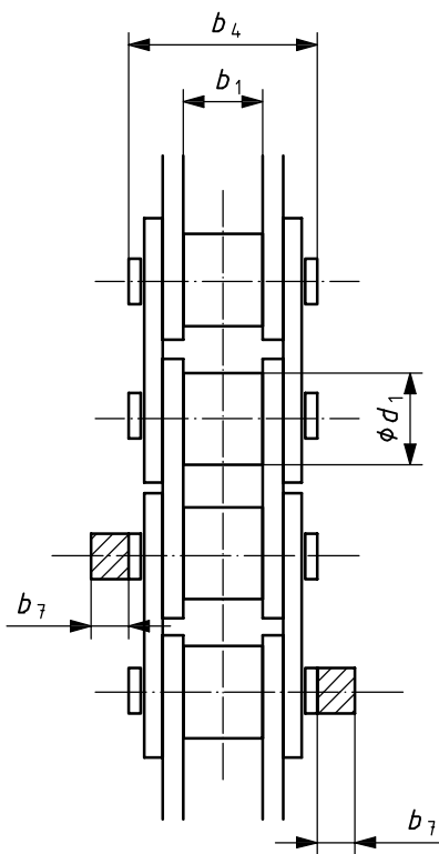
a) Roller chain
