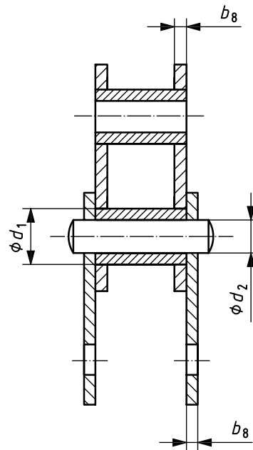
b) Bush chain
