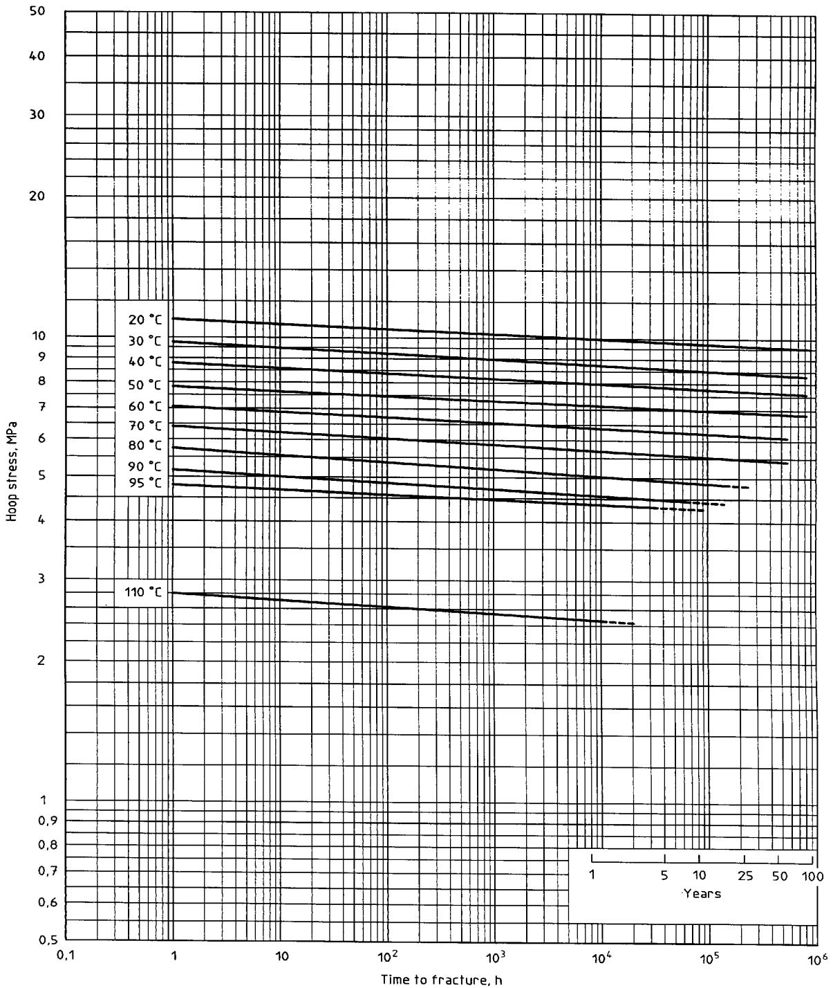
Figure 1 — Expected strength of crosslinked polyethylene (PE-X) pipes
