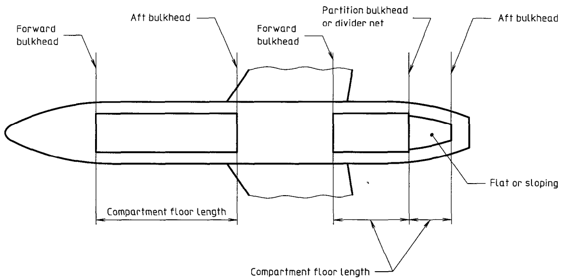
Figure 4 — Lower deck compartment usable length
