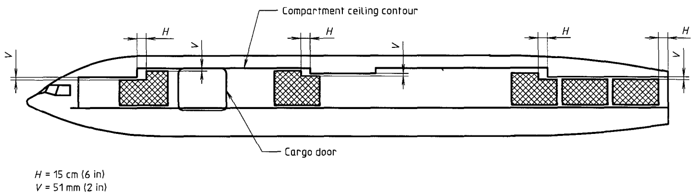
Figure 8 — Palletized cargo contour clearances
