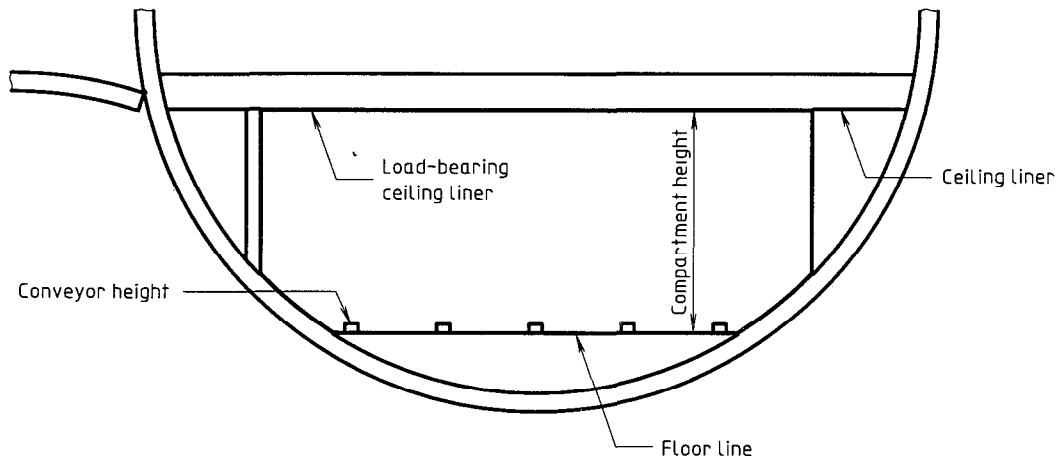
Figure 5 — Lower deck compartment usable height
