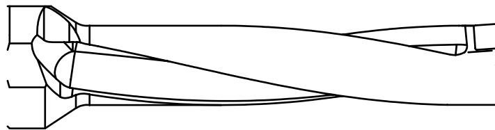
Figure A.50 — Layer 1 — Outer contour for assembled tool
