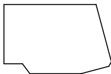
Figure A.34 — Layer NOCUT — Non-cutting contour for assembled tool
