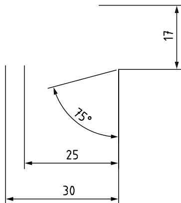
Figure A.33 — Layer 2 — Dimensioning for assembled tool
