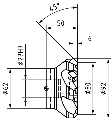
Figure A.12 — Tool component — All layers
