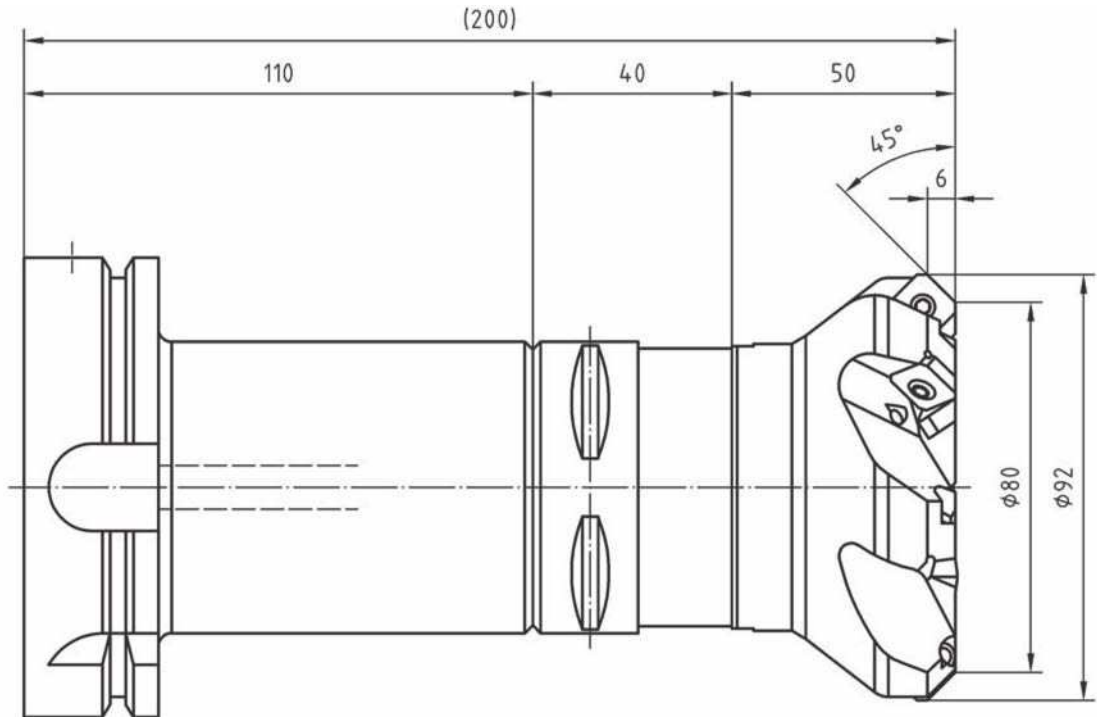
Figure 4 — Assembled tool — Illustration of Layers 1 to 11
