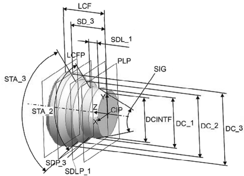
Figure 26 — Stepped countersinking tool — Revolved body of cutting part
