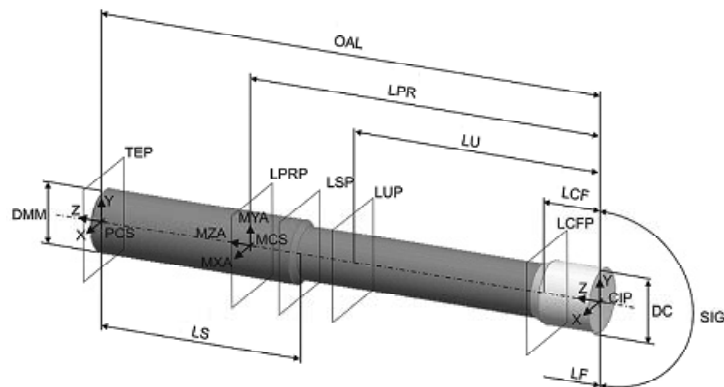
Figure 22 — Counterbore — Complete
