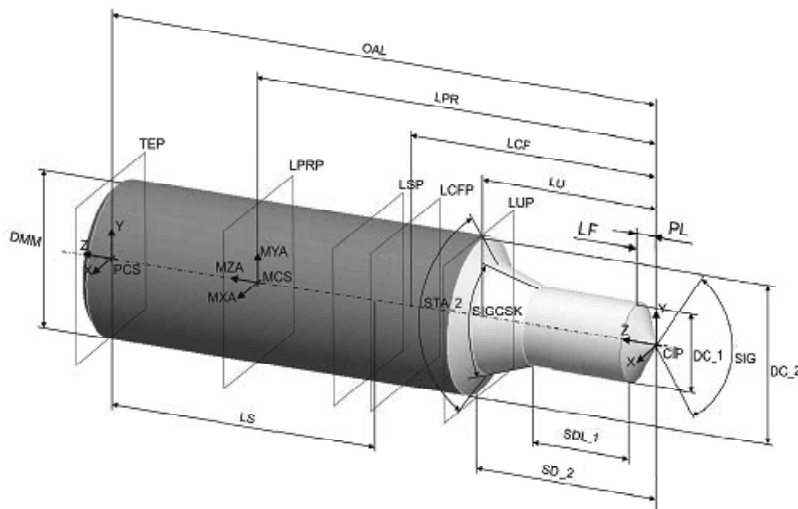
Figure 42 — Centre drill, style B — Complete
