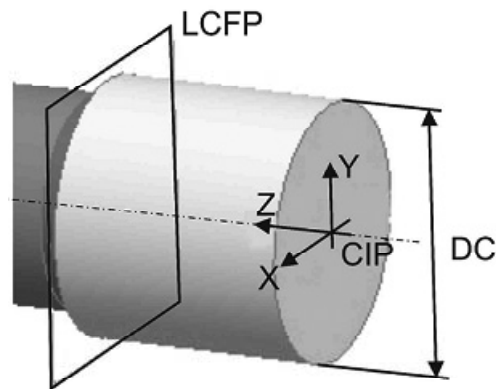
Figure 21 — Counterbore — Revolved body of cutting part
