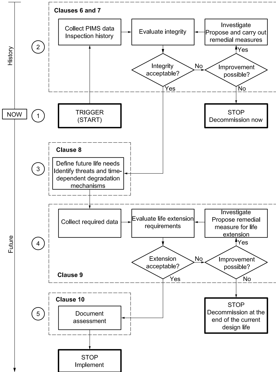
Figure 2 — Pipeline system life extension process
