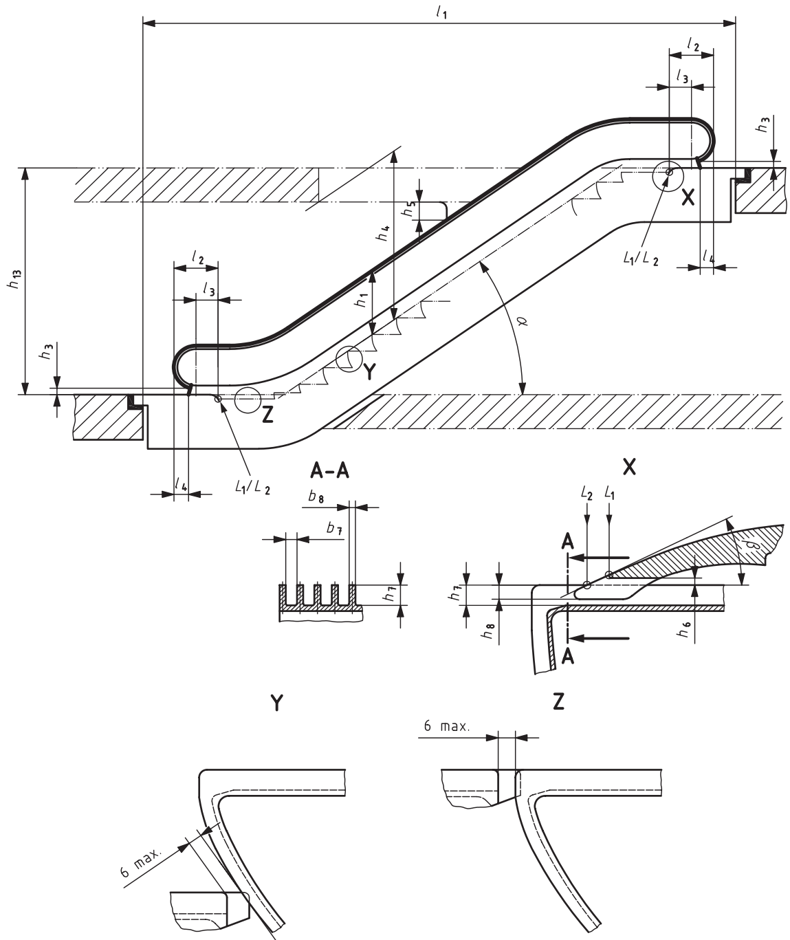
Figure A.2 — Escalator (elevation), principal dimensions (EN 115-1, Figure 2)
