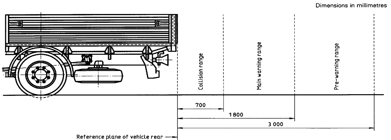
Figure 1 — Monitoring range of reversing detection device
