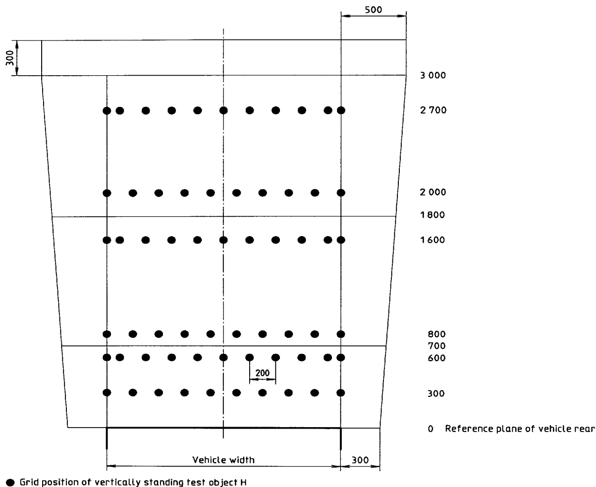
Figure 3 — Test 1 (plan view)
