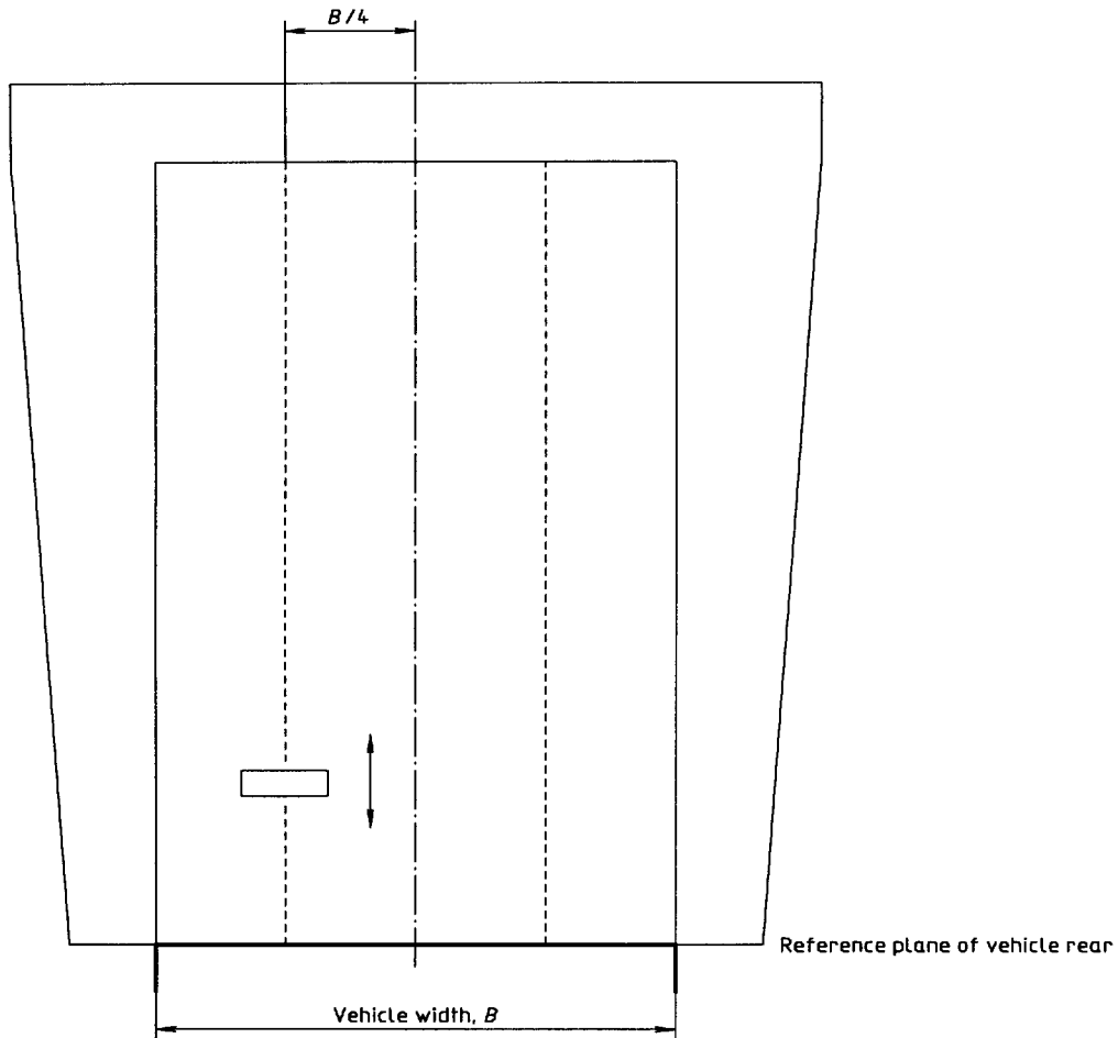
Figure 7 — Test 4 (plan view)
