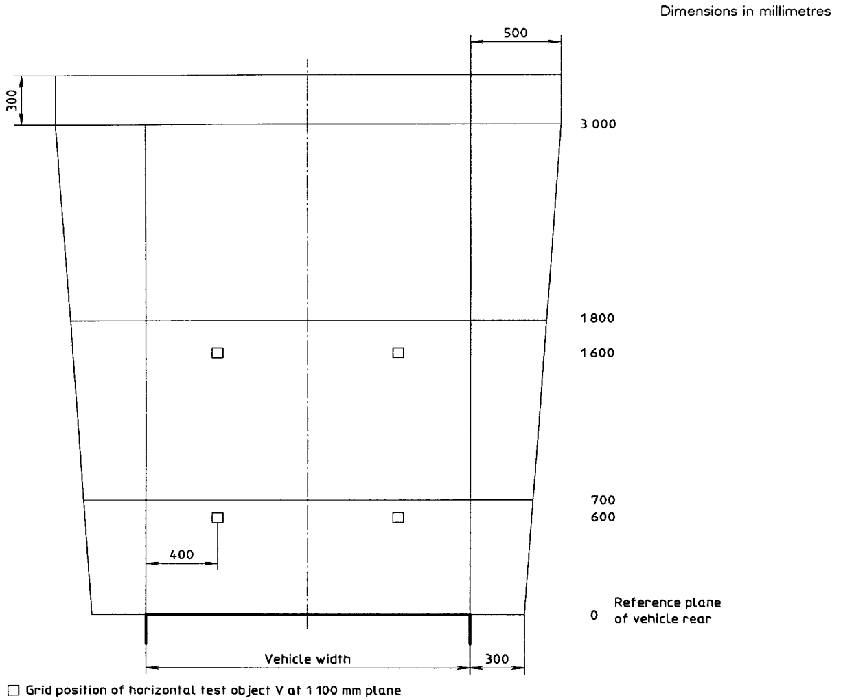
Figure 5 — Test 2 (plan view)
