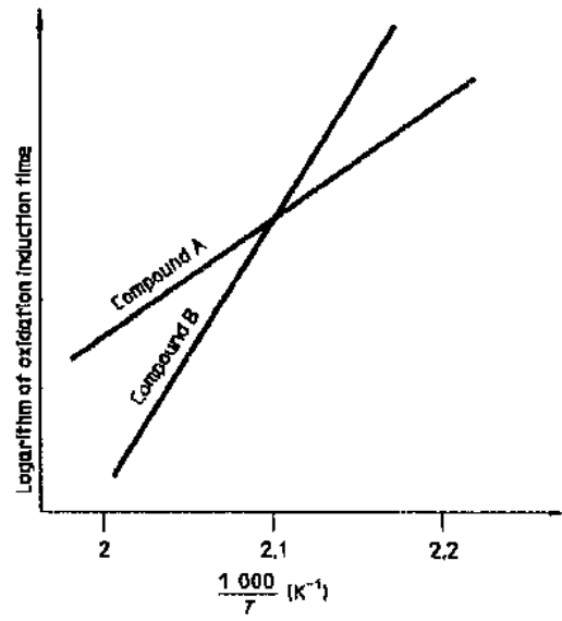
Figure 0.1 — Oxidation of two different stabilizer systems
