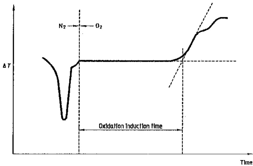
Figure 2 — Typical oxidative thermal stability curve for polyethylene
