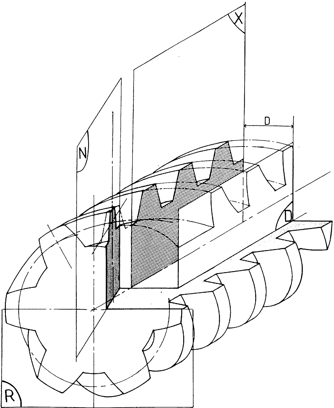
Figure 16 : Projection planes
