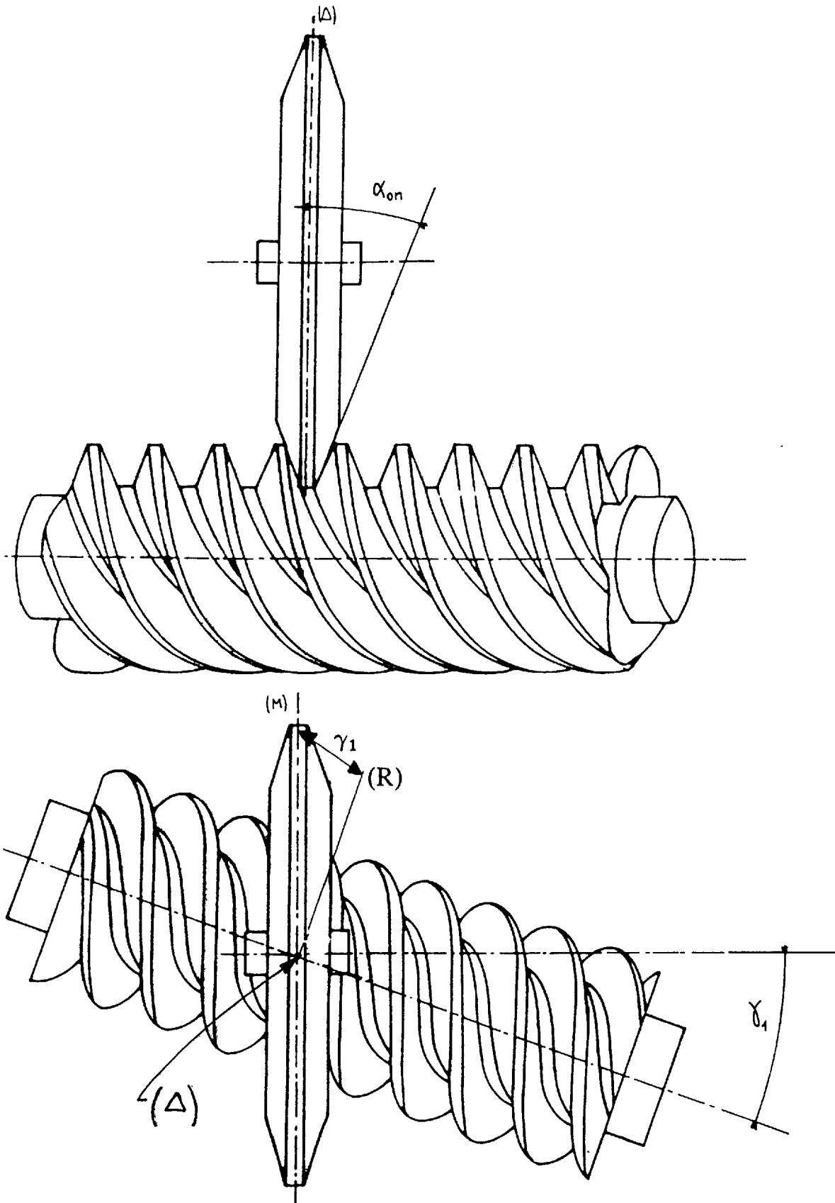
Figure 10 : Profile K - Machining method
